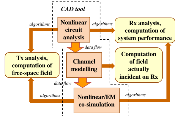
Fig. 17. CAD-based design flow for modern RF/microwave micro-systems.
