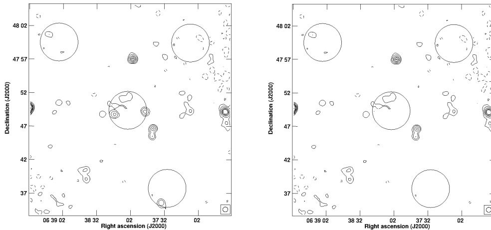
Fig. 2. Zwcl0634.1+4750 NVSS map; the contour levels are 0.66 \times (-1, 1, 2, 4, 6, 8, 10, 16, 32, 64) mJy \text{b}^{-1} . The 1\sigma level is 0.22 mJy \text{b}^{-1} . In both panels the region where we extracted the flux densities are shown (solid circles). The central region has a diameter of 1 Mpc and is centred on the centroid of the X-ray emission; the other three areas are the control fields. With the task BLANK we masked the discrete sources in the central region and the one that falls in the lower control field ( left panel ).
