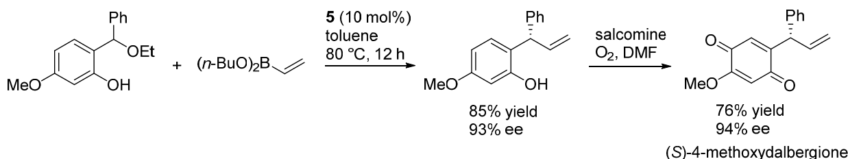
Scheme 25. Addition of vinylboronate and synthesis of ( S )-4-methoxydalbergione.
