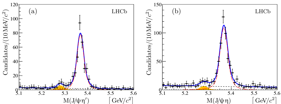
Figure 2. Mass distributions of (a) B_{(s)}^0 \rightarrow J/\psi\eta' and (b) B_{(s)}^0 \rightarrow J/\psi\eta candidates. The decays \eta' \rightarrow \eta\pi^+\pi^- and \eta \rightarrow \pi^+\pi^-\pi^0 are used in the reconstruction of J/\psi\eta' and J/\psi\eta candidates, respectively. The total fit function (solid blue) and the combinatorial background contribution (dashed black) are shown. The long-dashed red line represents the signal B_s^0 contribution and the yellow shaded area shows the B^0 contribution.
