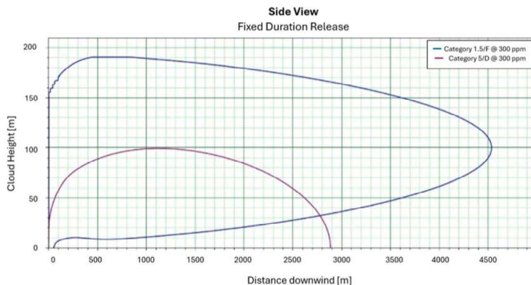
Figure 11. Cloud height of scenario S—dispersion on land.
