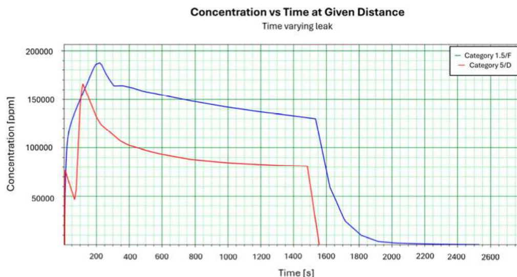
Figure 4. Scenario C dispersion on water—concentration vs time.
