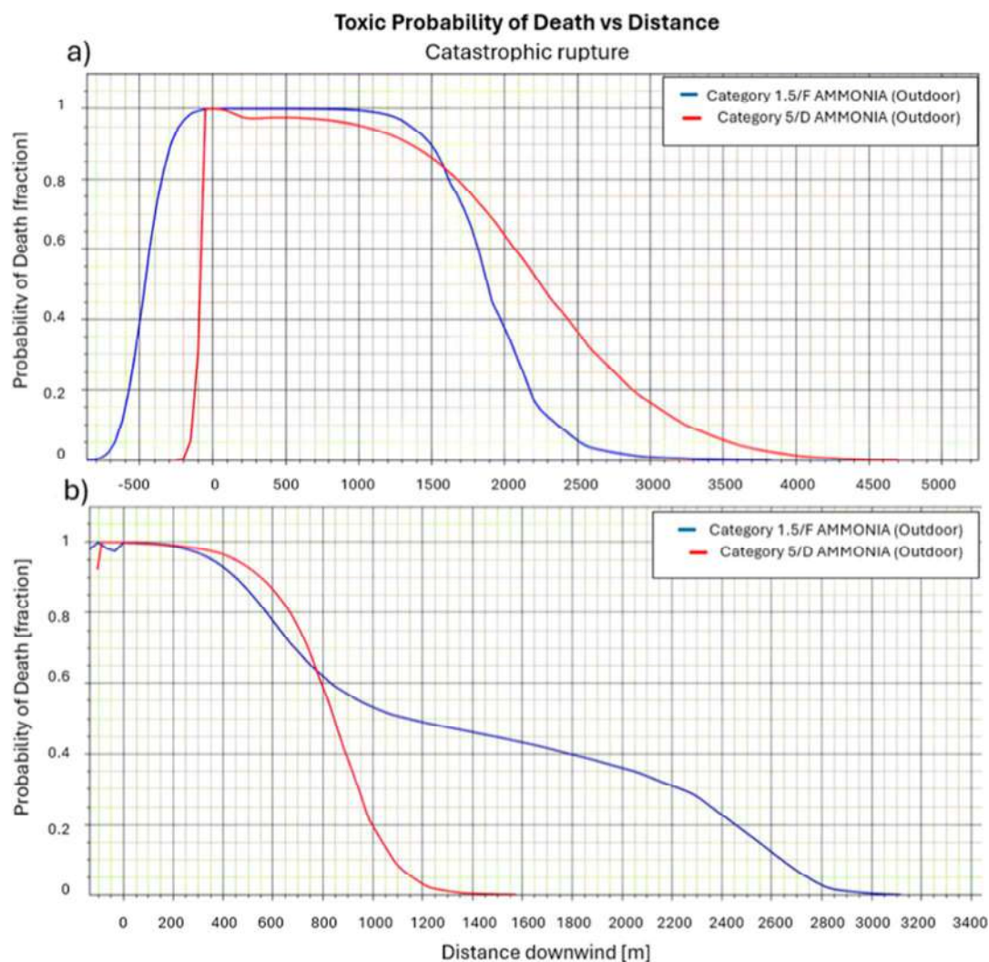
Figure 12. PoD—scenario L overwater unmitigated (a) and mitigated (b).
