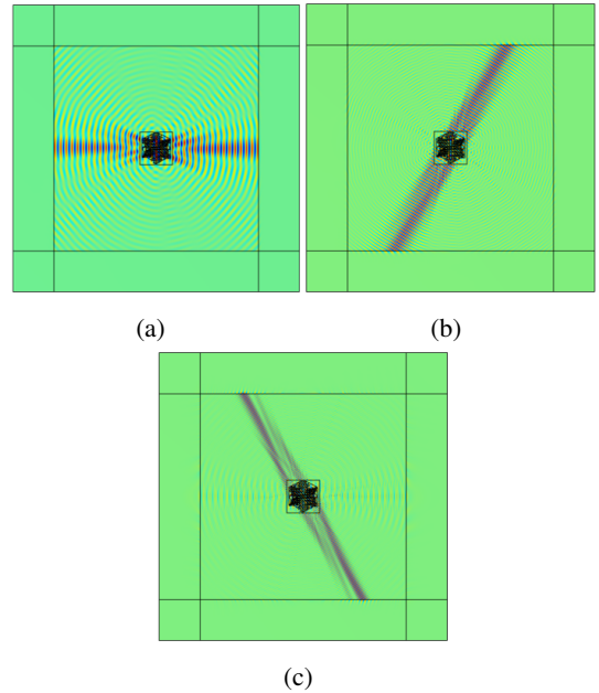
Fig. 3: Wavefields from Finite Element (FE) simulation at three different frequencies of 122 kHz, 168 kHz and 388 kHz propagating at 0^\circ , 60^\circ , and 120^\circ , respectively.
