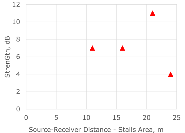
Fig. 11. Results of strength (G) in function of the receivers' distance.
