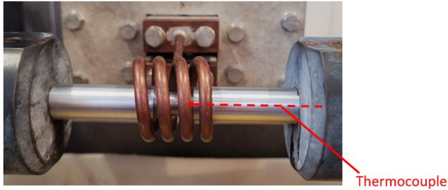
Fig. 2. Experimental setup for specimen heating using an induction copper coil. The thermocouple is positioned inside the axial hole near the gauge section, providing real-time temperature feedback for PID-controlled thermal regulation during torsion testing.
