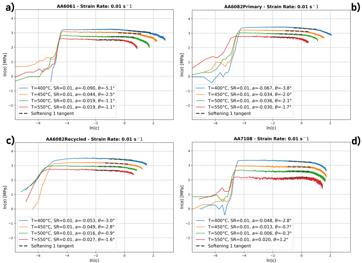
Fig. 8 Initial softening behavior (first 30% of post-peak data) for AA6061 (a), AA6082 Primary (b), AA6082 Recycled (c), and AA7108 (d) alloys at a strain rate of 0.01 s -1 . Linear regressions highlight the initial softening tangent (black dashed lines), with slope a and angle \theta reported for each temperature. Increasing temperature reduces the severity of early post-peak softening.
