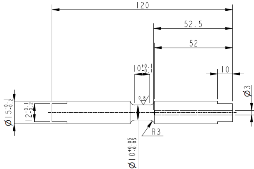
Fig. 1. Geometry of the solid cylindrical specimen used for hot torsion tests. The gauge section has a diameter of 10 mm and includes an axial hole (Ø3 mm, length 52.5 mm) for thermocouple placement, enabling accurate temperature monitoring during deformation.
