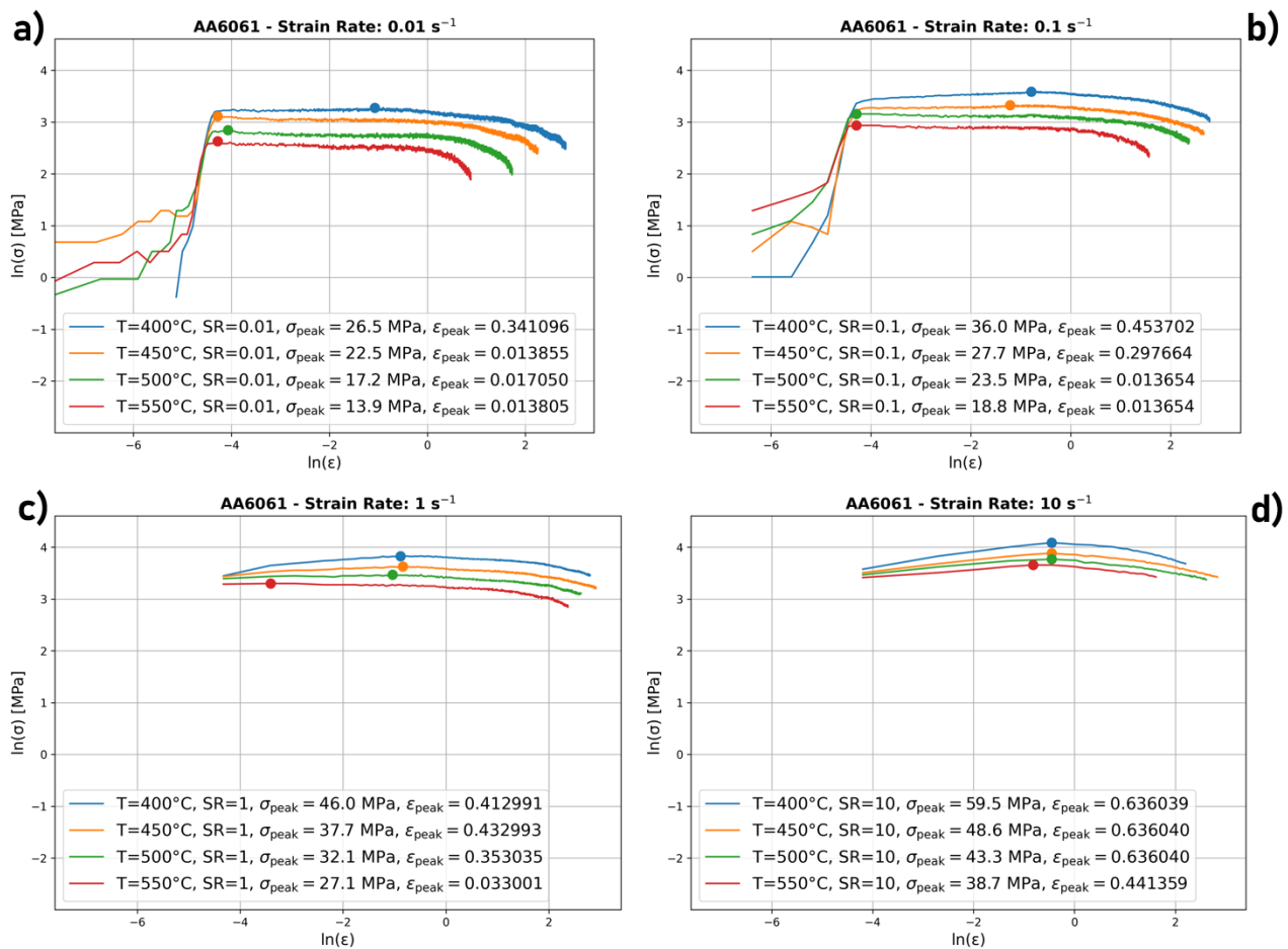
Fig. 7 Hot torsion flow curves for AA6061 alloy in the \ln\sigma – \ln\epsilon domain at different temperatures ( 400 – 550^\circ\text{C} ) and strain rates ( 0.01 (a), 0.1 (b), 1 (c), 10 \text{ s}^{-1} (d)). Symbols indicate peak stress ( \sigma_{\text{peak}} ) and corresponding strain ( \epsilon_{\text{peak}} ). Post-peak softening behavior is evident, with thermal softening dominating at low strain rates and strain-rate hardening prevailing at high strain rates.
