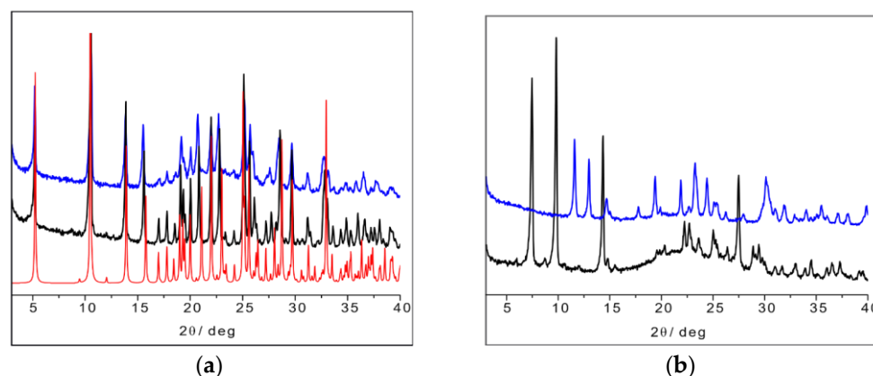
Figure 16. (a) L- \text{His}_2 \cdot \text{Ag} (TIGHEY) [56] calculated pattern from database (in red), experimental XRPD pattern from slurry synthetic procedure of L- \text{His}_2 \cdot \text{Ag} (in black), and DL- \text{His}_2 \cdot \text{Ag} (in blue); (b) experimental XRPD pattern from slurry of L- \text{His} \cdot \text{Ag} (in black) and DL- \text{His} \cdot \text{Ag} (in blue).
