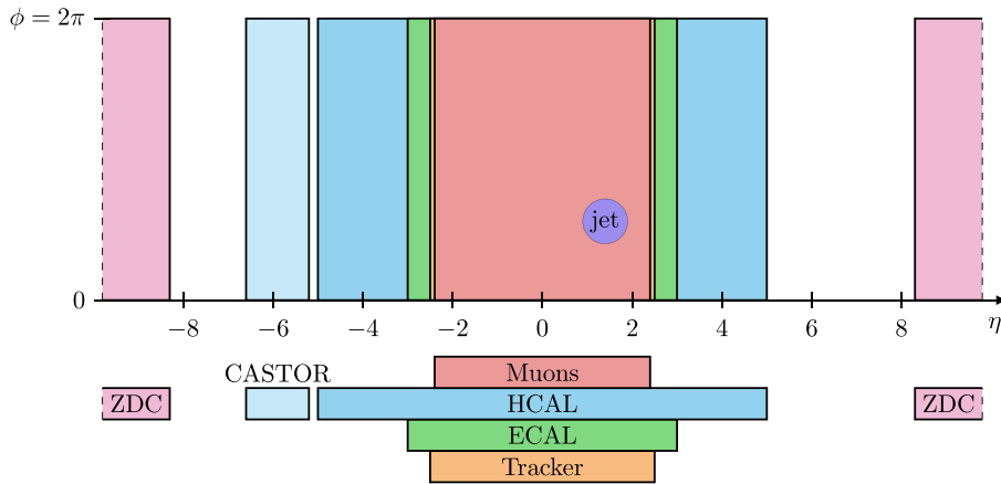
Fig. 2. A simplified sketch of the acceptance in \eta and \phi for the tracking, calorimetry (ECAL, HCAL, CASTOR, and ZDC) and muon identification (“Muons”) components of the CMS detector. In the lower section, the central elements (that is, excluding ZDC and CASTOR) are arranged based on their proximity to the beam, with the tracker being the closest element of the central detectors, and the muon detectors positioned farthest away. The size of a jet cone with R = 0.5 (to be discussed in Section 2.10) is also depicted for illustration. Source: Figure adapted from Ref. [4].
