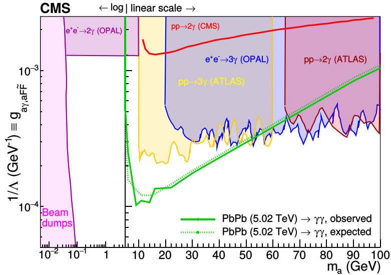
Fig. 111. Exclusion limits at 95% CL in the ALP-photon coupling g_{a\gamma} vs. ALP mass m_a plane, for the operators a\tilde{F}/4\Lambda assuming ALP coupling to photons only, derived in Refs. [587,593] from measurements at beam dumps [594], in e^+e^- collisions at LEP 1 [593] and LEP 2 [595], and in pp collisions at the LHC [574,596,597], and compared to the limits obtained from Ref. [548]. Source: Figure adapted from Ref. [548].
