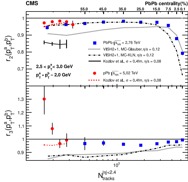
Fig. 39. The p_T -dependent factorization ratios, r_2 and r_3 , as functions of event multiplicity in pPb and PbPb collisions. The lines represent different hydrodynamics calculations.
