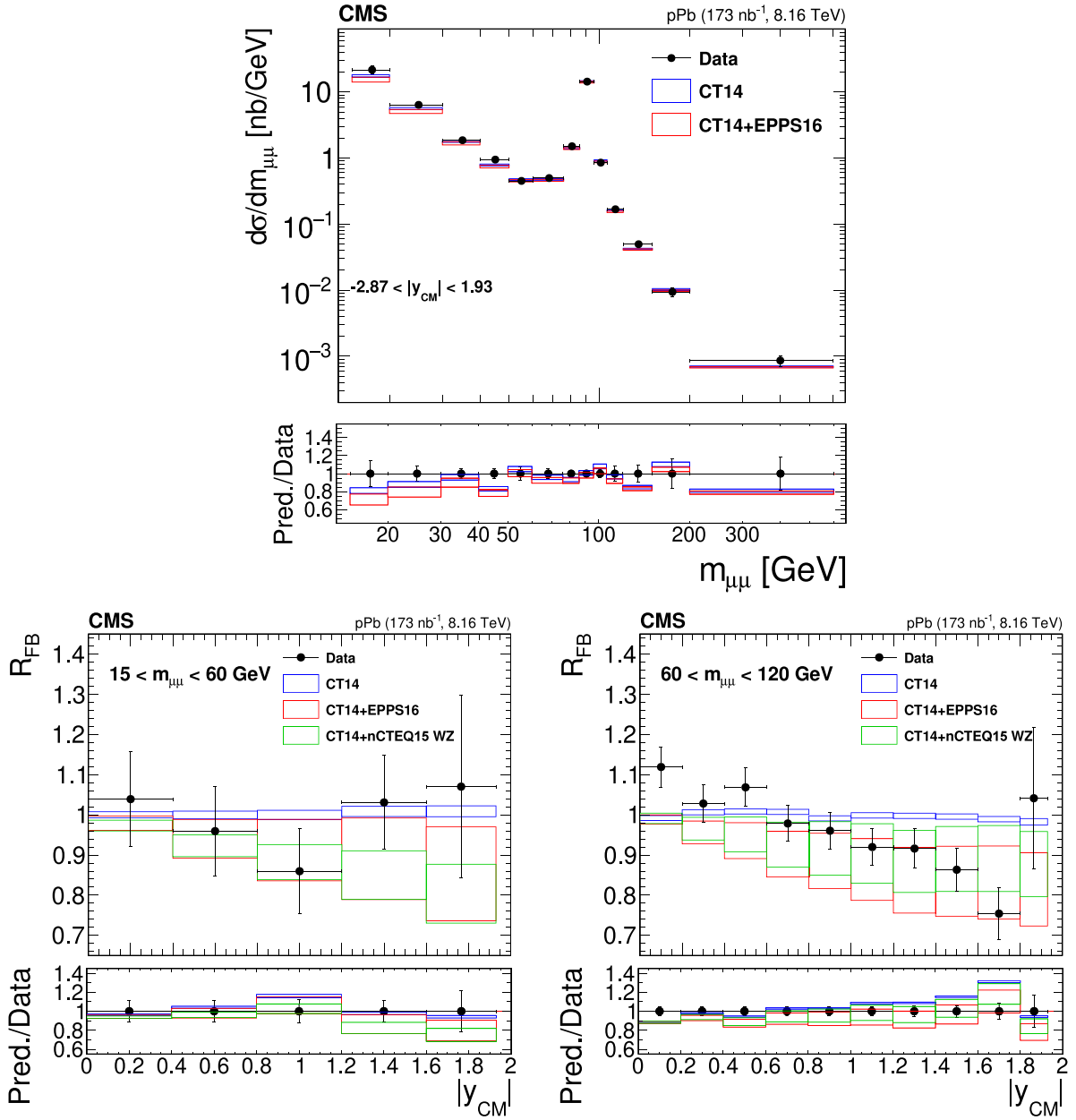
Fig. 14. Differential cross section for the Drell–Yan process measured in the muon channel as a function of the dimuon invariant mass (upper) and the forward–backward ratios for 15 < m_{\mu^+\mu^-} < 60 GeV (lower left) and 60 < m_{\mu^+\mu^-} < 120 GeV (lower right). Error bars represent the total measurement uncertainty. Theory predictions from the POWHEG NLO generator using the CT14 PDF (blue), or the CT14+EPPS16 (red) or CT14+nCTEQ15WZ (green) nPDF sets are shown. The standard deviation of the nPDF uncertainties are shown by the boxes. Ratios of theory predictions over data are shown in the lower panels. Source: Figure adapted from Ref. [166].
