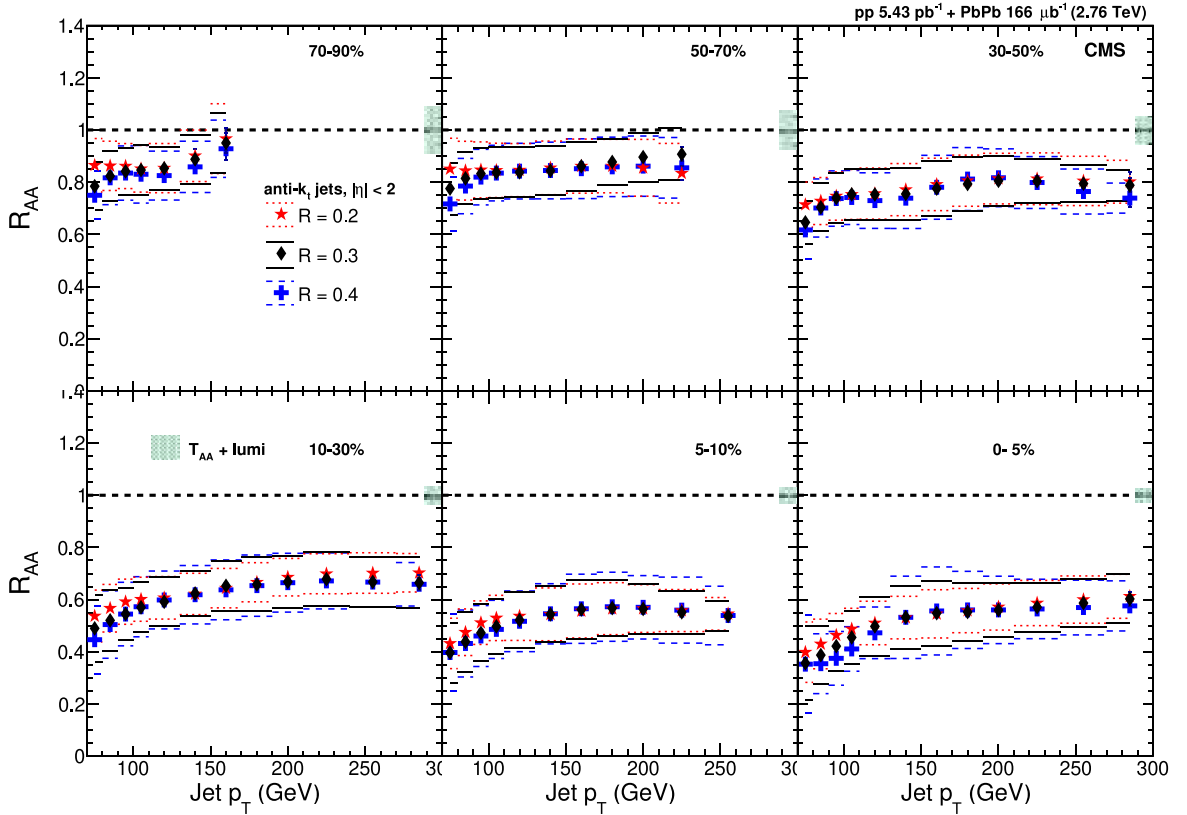
Fig. 55. Inclusive jet R_{AA} plotted as a function of the jet p_T for |\eta| < 2.0 . Each panel corresponds to a different centrality class (upper left) 70%–90%, (upper middle) 50%–70%, (upper right) 30%–50%, (lower left) 10%–30%, (lower middle) 5%–10%, and (lower right) 0%–5%. Results for three jet distance parameters, R = 0.2, 0.3 , and 0.4 , are overlaid as red stars, black diamonds, and blue crosses, respectively. Vertical bars (typically smaller than the markers) represent the statistical uncertainty, while horizontal bars around each point are the nonglobal systematic uncertainties. Finally, the combined global systematic uncertainty coming from T_{AA} and the integrated luminosity measurement is plotted as a shaded green bar on the horizontal black-dashed unity line.
