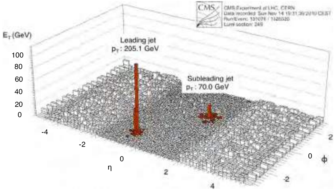
Fig. 52. An “unrolled” calorimeter display of energy deposition in an event containing an unbalanced dijet pair in a \sqrt{s_{\text{NN}}} = 2.76 TeV PbPb collision, as recorded by the CMS detector in 2010. The tower-by-tower transverse energy sum combining the measurement in electromagnetic and hadronic calorimeters is plotted as a function of \eta and \phi . The fully corrected transverse momenta of the unbalanced dijet pair are labeled and their position in \eta - \phi indicated with the red-highlighted constituent towers.
