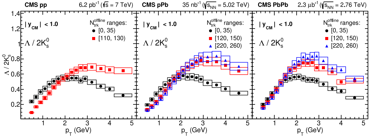
Fig. 87. Ratios of p_T spectra for \Lambda/2K_S^0 in the center-of-mass rapidity range |y_{\text{cm}}| < 1.0 for pp collisions at \sqrt{s} = 7 TeV (left), pPb collisions at \sqrt{s_{\text{NN}}} = 5.02 TeV (middle), and PbPb collisions at \sqrt{s_{\text{NN}}} = 2.76 TeV (right). Two (for pp) or three (for pPb and PbPb) representative multiplicity intervals are presented.
