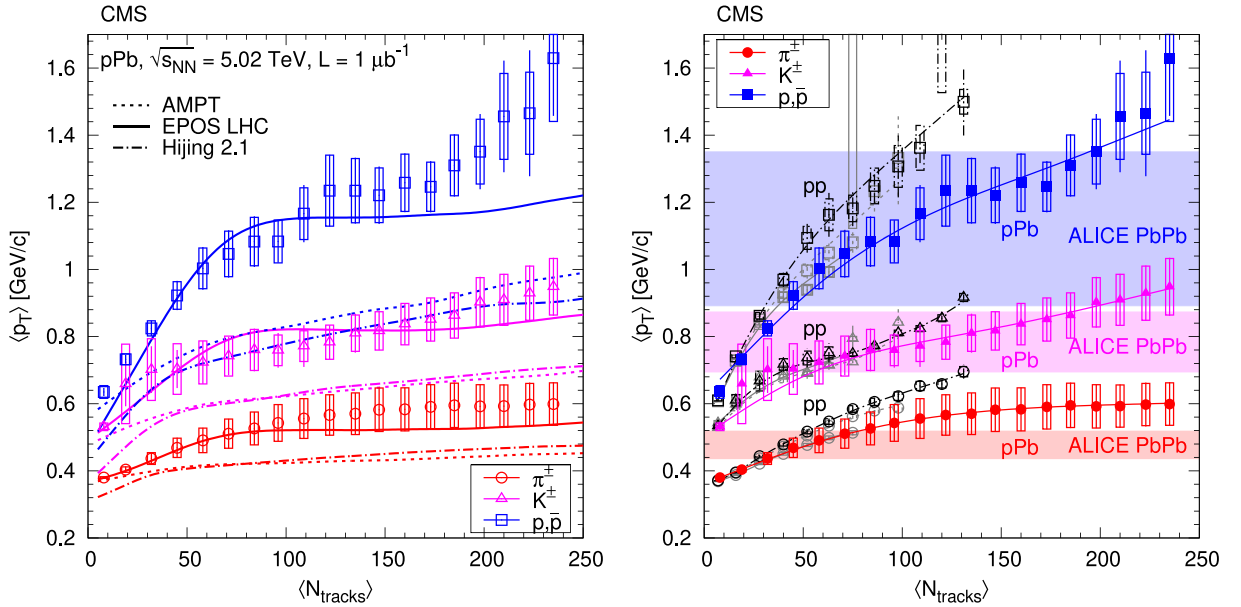
Fig. 86. Average transverse momentum of identified charged hadrons in the range |\eta| < 2.4 , for pp collisions (open symbols) at several energies [502] and for pPb collisions (filled symbols) at \sqrt{s_{NN}} = 5.02 TeV. Left: Results compared to predictions from event generators. Right: Comparison of pp, pPb, and PbPb data. The ranges of \langle p_T \rangle values measured by ALICE in various centrality PbPb collisions at \sqrt{s_{NN}} = 2.76 TeV [503] are indicated with horizontal bands.
