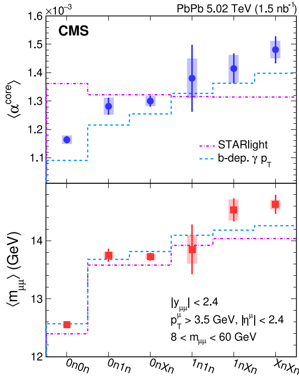
Fig. 103. Neutron multiplicity dependence of the (upper) average acoplanarity \langle \alpha^{core} \rangle and (lower) average invariant mass \langle m_{\mu\mu} \rangle of \mu^+\mu^- pairs in ultraperipheral PbPb collisions at \sqrt{s_{NN}} = 5.02 TeV. The vertical lines on data points depict the statistical uncertainties while the systematic uncertainties of the data are shown as shaded areas. The dot-dashed line shows the STARLIGHT MC prediction and the dashed line corresponds to the LO QED calculation of Ref. [571]. The calculation incorporating Sudakov radiative corrections is also compared to data in Ref. [218], leading to an overall better agreement. Source: Figure adapted from Ref. [218].
