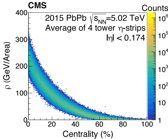
Fig. 10. Distribution of \rho , the UE energy per unit area, as a function of centrality, found using the central- \eta strip of PF pseudotowers. Source: Figure adapted from Ref. [142].
