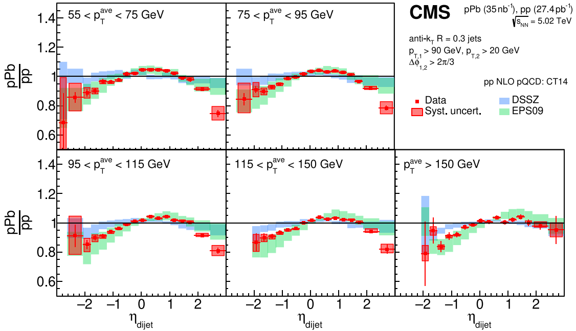
Fig. 16. The ratio of the dijet \eta spectra for pPb and pp data in a selection of p_T^{\text{ave}} ranges. Theoretical predictions are from the NLO pQCD calculations of DSSZ [175] and EPS09 [176] are shown. Red boxes and bars indicate the systematic and statistical uncertainties in data, respectively. Green and blue boxes represent nPDF uncertainties. Source: Figure adapted from Ref. [177].
