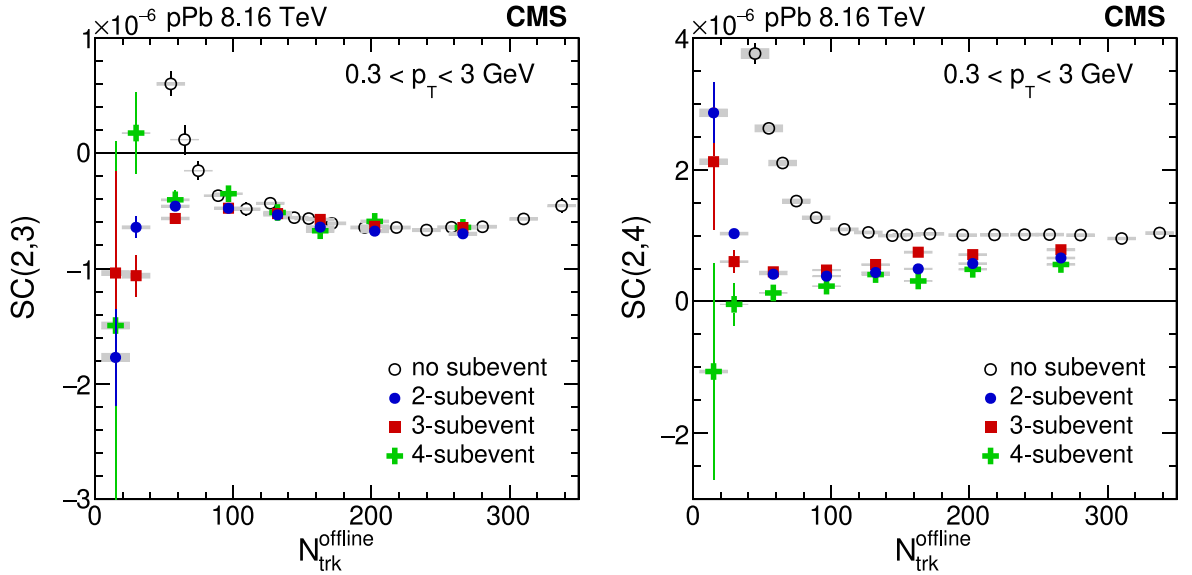
Fig. 91. The SC(2, 3) (left panel) and SC(2, 4) (right panel) distributions as functions of N_{\text{trk}}^{\text{offline}} from methods using no (open black circles), 2 (full blue circles), 3 (red squares), and 4 (green crosses) subevents for pPb at 8.16 TeV. Statistical and systematic uncertainties are shown by vertical bars and shaded boxes, respectively.
