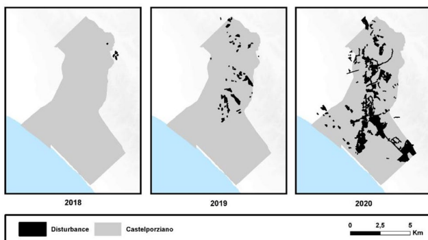
Fig. 2 Disturbance maps of 2018, 2019, and 2020
