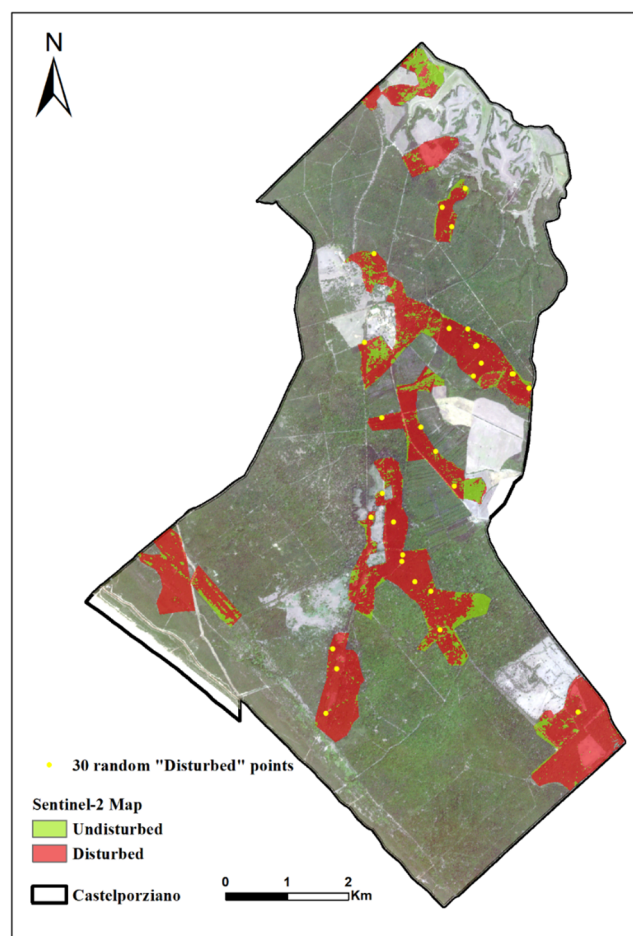
Fig. 5 30 random “Disturbed” points used to calculate the MTL
