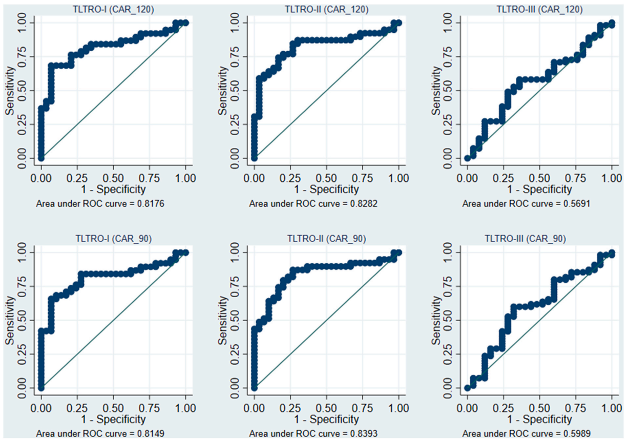
Fig. A4. ROC curves based on equation (5). This figure shows the area under the ROC curve for a probit model where the dependent variable is equal to one if a bank received funding under one of the three waves of the TLTRO program, TLTRO-I, TLTRO-II, and TLTRO-III. The independent variable is the estimated bank-level CAR(-1,1) for the corresponding announcement. “CAR 120 ” (“CAR 90 ”) denotes that the estimation window is based on 120 (90) trading days.
