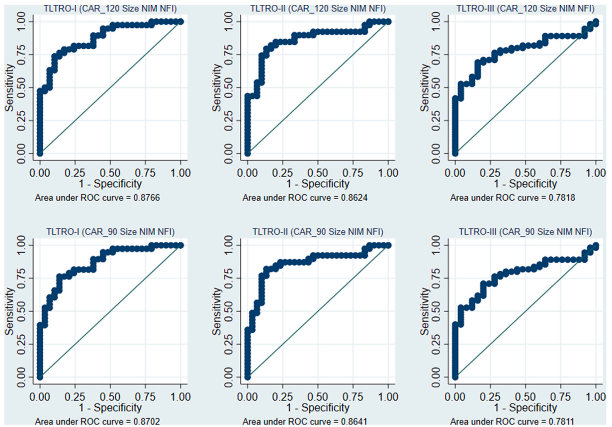
Fig. A5. ROC curves with control variables (equation (6)). This figure shows the area under the ROC curve for a probit model where the dependent variable is equal to one if a bank received funding under one of the three waves of the TLTRO program, TLTRO-I, TLTRO-II, and TLTRO-III. The main independent variable is the estimated bank-level CAR(-1,1) for the corresponding announcement. The controls are: Size , NIM , and NFI . “CAR_120” (“CAR_90”) denotes that the estimation window is based on 120 (90) trading days.
