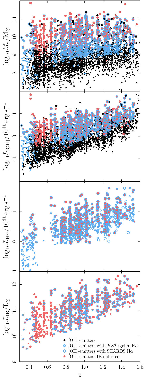
Figure 4. Stellar masses, [O II] luminosities, H\alpha luminosities (from HST /grism and SHARDS data; only H\alpha detections at \text{SNR} > 3 ), and total IR luminosities (see Section 2.5) of the sample of SHARDS [O II] emitters as a function of redshift. The H\alpha luminosities are corrected for [\text{N II}]\lambda\lambda 6568.1, 6583.6 contamination (see Section 6.1). The size of the data points scales with the stellar mass: small, medium, and large for \log_{10} M_*/M_\odot < 9 , 9 < \log_{10} M_*/M_\odot < 10 , and \log_{10} M_*/M_\odot > 10 , respectively.
