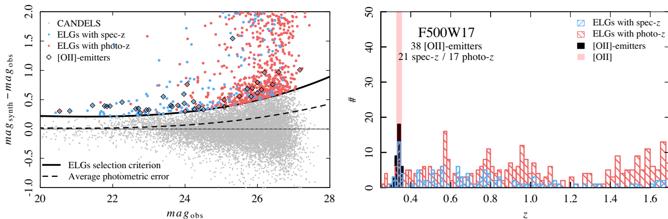
Figure 2. Left panel: Colour–magnitude diagram showing ELG candidates in SHARDS filter F500W17. Colour is defined as the difference between the synthetic and the observed magnitudes. The colour threshold which defines the locus of ELGs is marked with a black continuous line. The colour equal to zero is marked with a horizontal thin dashed black line. The dashed curve represent the average photometric error. Right panel: Redshift distribution of the ELG candidates throughout the redshift range in which [O II] falls within the wavelength range over which SHARDS extends. The vertical coloured line marks the redshift that shifts the [O II] line into the SHARDS F500W17 filter. The blue (red) histogram displays the distribution of galaxies with spectroscopic (photometric) redshifts. The black histogram shows the distribution of the 38 [O II] emitters detected in the F500W17 band. Appendix A includes analogous figures for the rest of the SHARDS filters.
