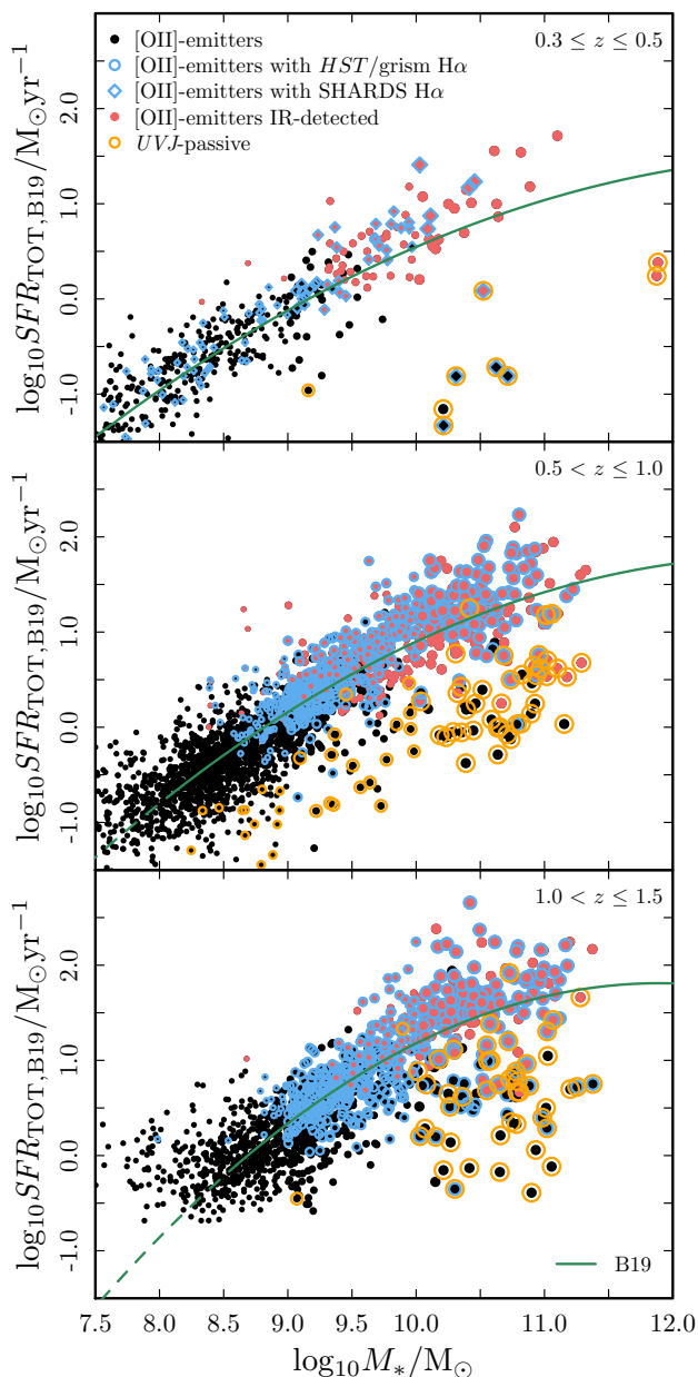
Figure 6. SFR_{\text{TOT}} versus M_* relation for the [O II] emitters split up in three increasing z bins (top, middle and bottom panels). The SFR_{\text{TOT}} refers to the SFR_{\text{TIR}} + SFR_{\text{UV}} for those galaxies IR-detected, and SFR_{\text{UV,corr}} otherwise (see B19 for details). Symbols as in Fig. 3. UVJ passive galaxies are highlighted with an orange circle. The green lines represent the main sequences fitted by B19 to samples of galaxies selected as star forming in the UVJ diagram. The relations are extended beyond the stellar mass completeness level using dashed lines.
