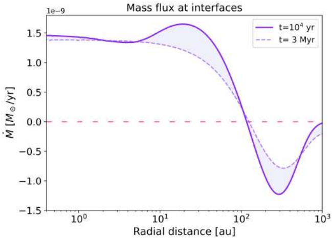
Fig. 5. Radial profiles of the mass accretion flux in the disc midplane in units of solar masses of gas per year. The plot shows the mass flux computed at the edges of each grid point at t = 10^4 \text{ yr} (solid curve) and t = 3 \text{ Myr} (dashed curve), corresponding to the beginning and the end of our simulations, respectively. The accretion flux is positive up to about 120 au and then becomes negative. A positive (negative) accretion flux indicates gas transport towards (away from) the star, which is consistent with the predictions of viscous evolution.
