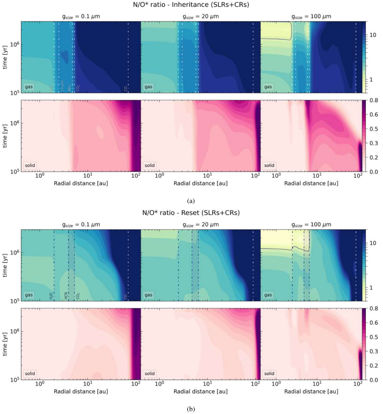
Fig. B.3: Same as Fig. 11 for the inheritance (panel a) and reset (panel b) scenarios with high ionisation.
