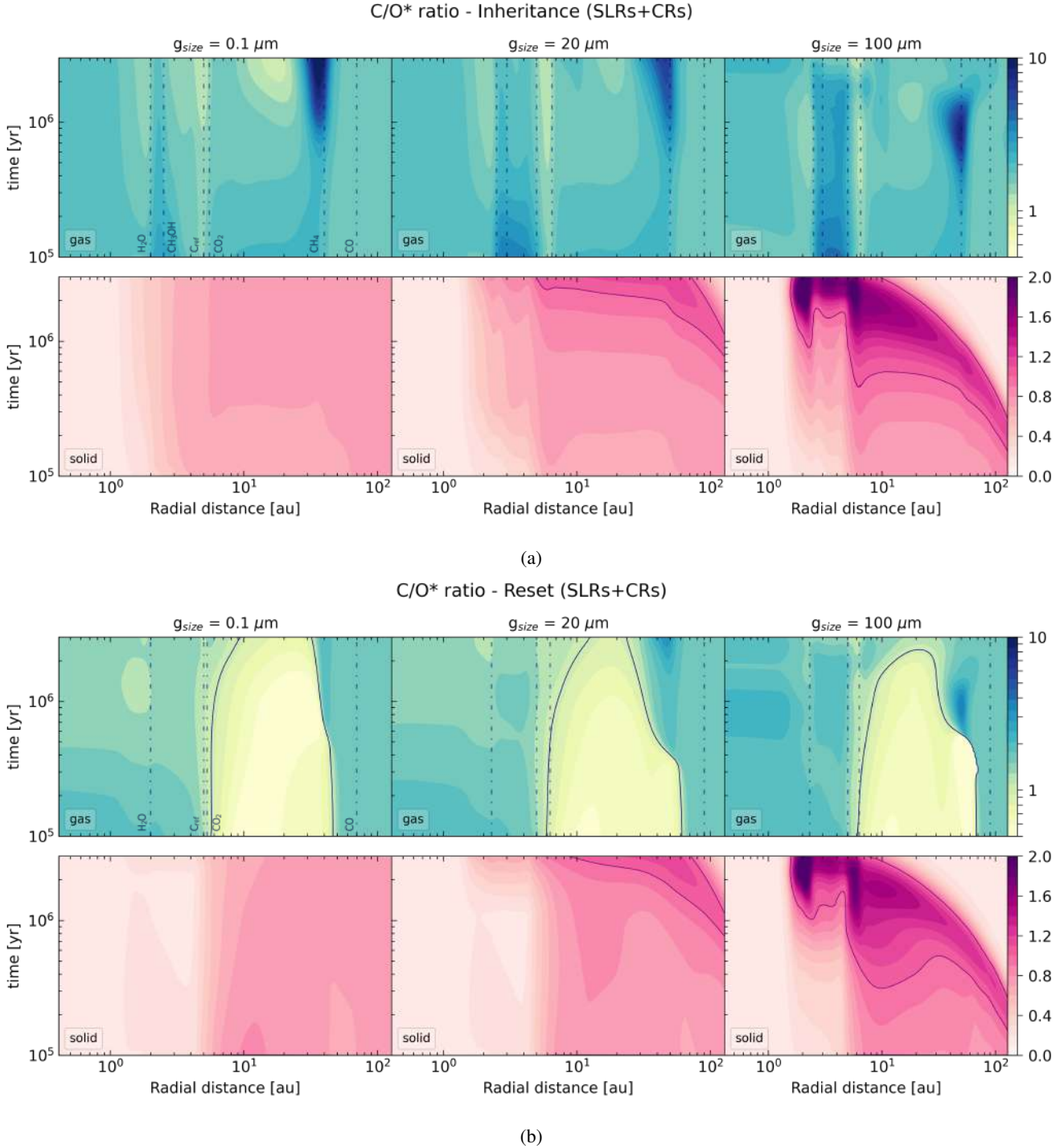
Fig. B.1: Same as Fig. 8 for the inheritance (panel a) and reset (panel b) scenarios with high ionisation.
