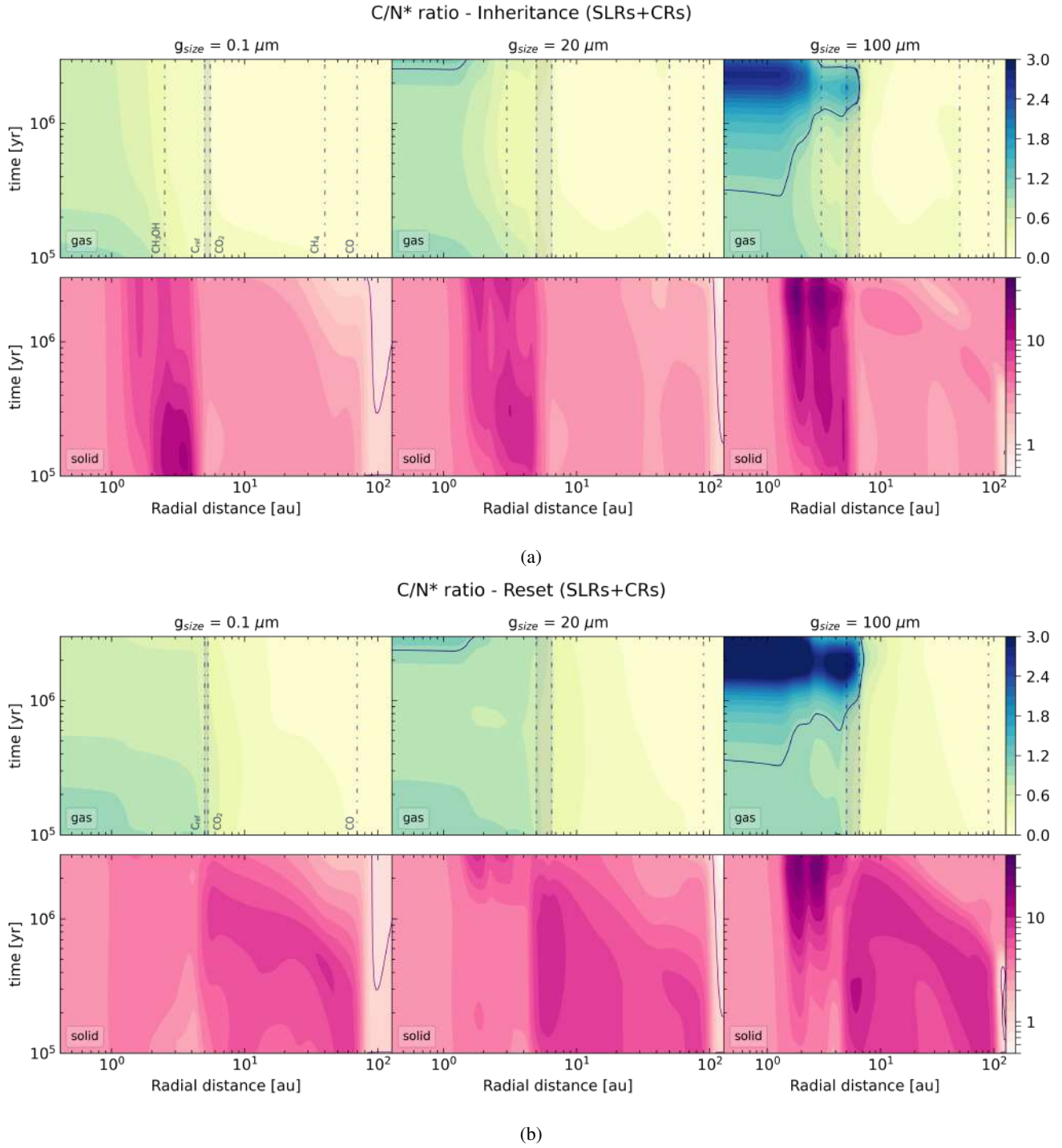
Fig. B.2: Same as Fig. 10 for the inheritance (panel a) and reset (panel b) scenarios with high ionisation.
