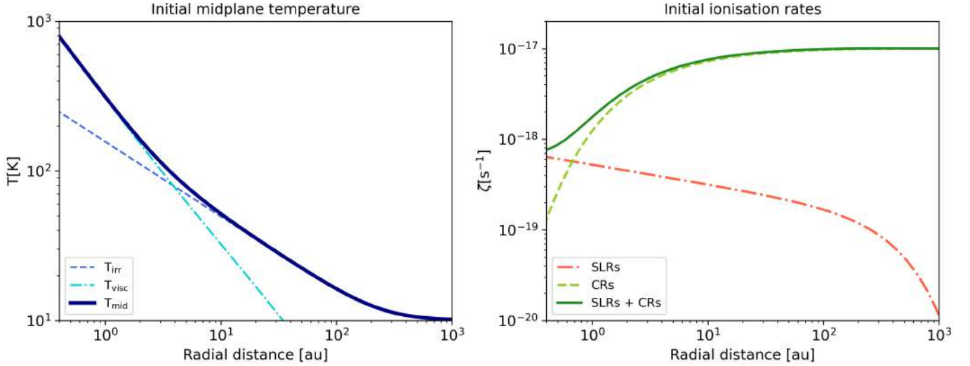
Fig. 2. Left: initial radial profile of the midplane temperature (solid) together with the contributions of stellar irradiation (dashed) and viscous heating (dash-dotted). The temperature reaches a minimum value of 10 K in the outer disc. Right: initial ionisation profiles in the midplane. The orange (dash-dotted) curve indicates the contribution of SLRs and characterises the ionisation environment in the low scenario. The green (solid) curve shows the total ionisation taking into account an additional contribution from CRs (light green curve) and characterises the ionisation environment in the high scenario.
