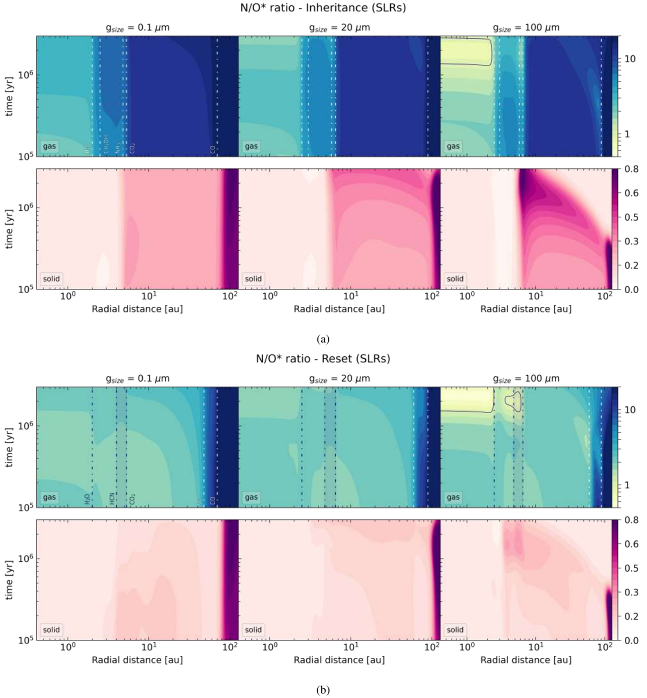
Fig. 11. N/O ratio in the disc as a function of distance and time for the inheritance (panel a) and reset (panel b) scenarios with low ionisation. In each panel, the top row represents the gas phase, while the bottom row shows the solid phase (including rocks, ice mantles, and refractory organic carbon). All values are normalised to the stellar N/O ratio ( \sim 0.14 ), with normalisation indicated by the superscript *. The dark contour represents a value of 1, corresponding to the stellar ratio. Vertical lines indicate the approximate locations of key snowlines at 2 Myr. Molecules are labelled only in the top-left plot of each panel but follow the same order in the other plots. For clarity, the \text{NH}_3 snowline in the reset scenario is not shown but lies within the shaded region between the HCN and \text{CO}_2 snowlines.
