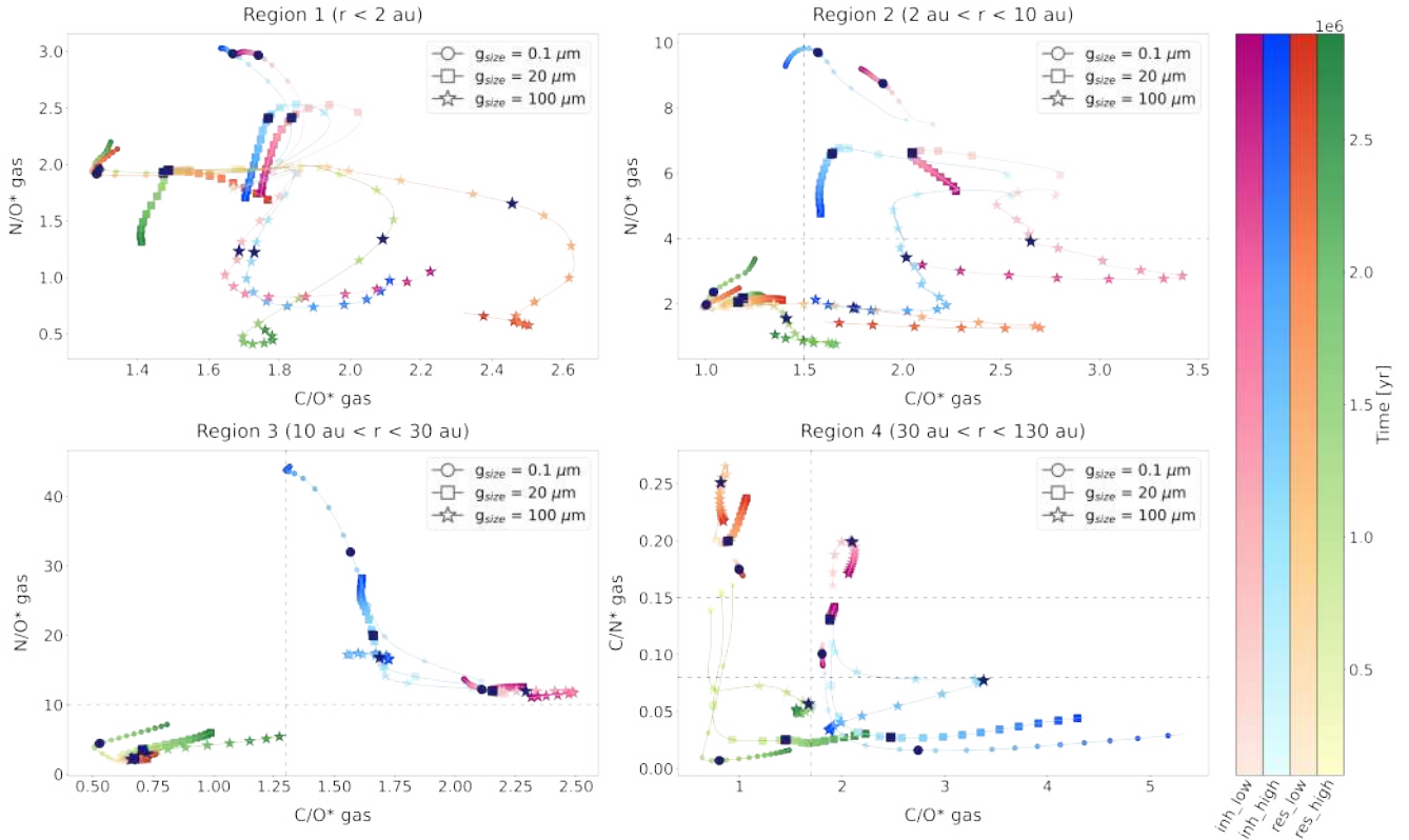
Fig. 12. Evolutionary tracks of the elemental ratios over 3 Myr across all considered scenarios. Ratios are shown in pairs across four key compositional regions: within the \text{H}_2\text{O} snowline (region 1, top-left), between the \text{H}_2\text{O} and \text{CO}_2 snowlines (region 2, top-right), between the \text{CO}_2 and \text{CH}_4 snowlines (region 3, bottom-left), and beyond the \text{CH}_4 snowline (region 4, bottom-right). Values represent gas-phase elemental ratios, calculated from total elemental abundances averaged over the radial extent of each region and weighted by the surface density of the gas. The colour bars indicate the four chemical scenarios, with time progressing from lighter to darker shades. The three different markers represent the selected grain sizes and are placed along each track every 200 000 yr. The dark marker on each track denotes 1 Myr. Dashed grey lines highlight regions of the parameter space where pairwise comparisons of the elemental ratios provide constraints on specific scenarios or subsets of scenarios.
