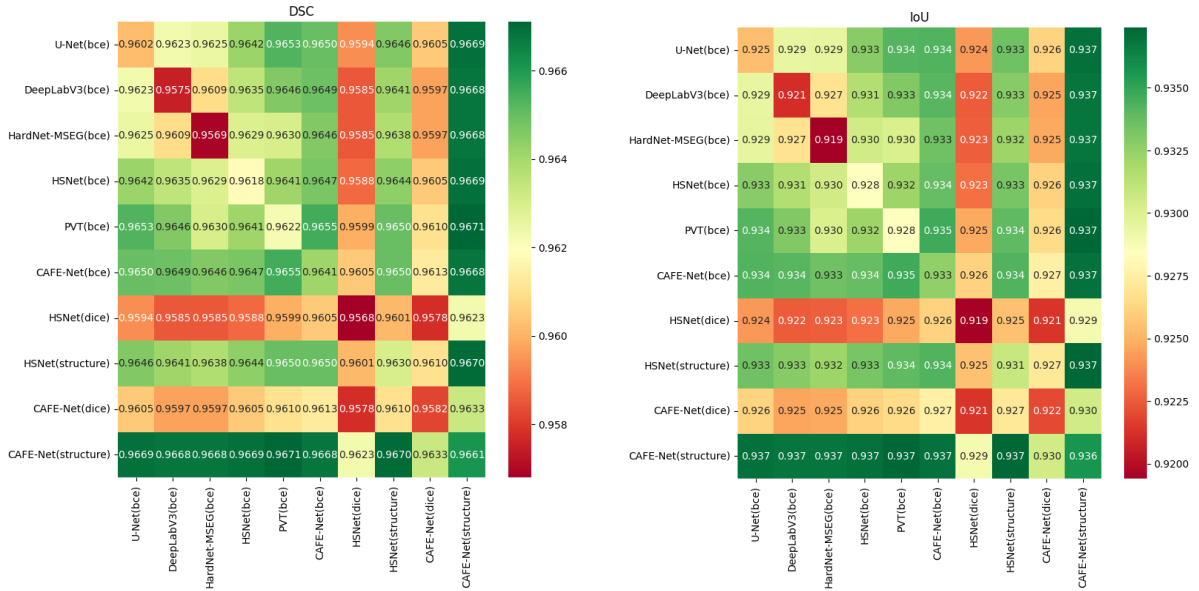
(a) DSC
