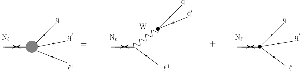
Fig. 2. Feynman diagrams for the decay of a heavy composite Majorana neutrino to lq\bar{q}' .
