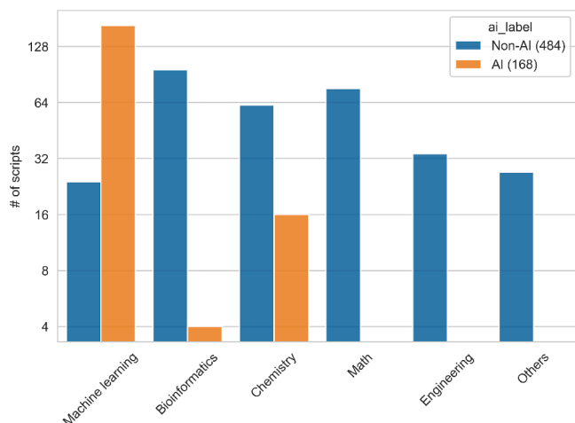
Fig. 3. Distribution of the job script domain , divided by the ai label.
