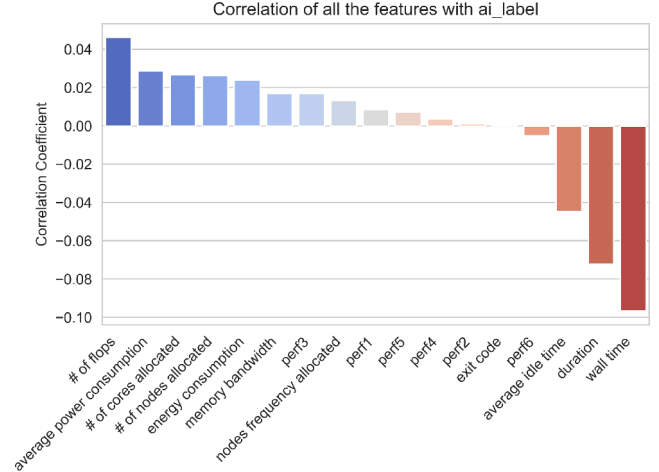
Fig. 7. Feature correlation with the ai_label .
