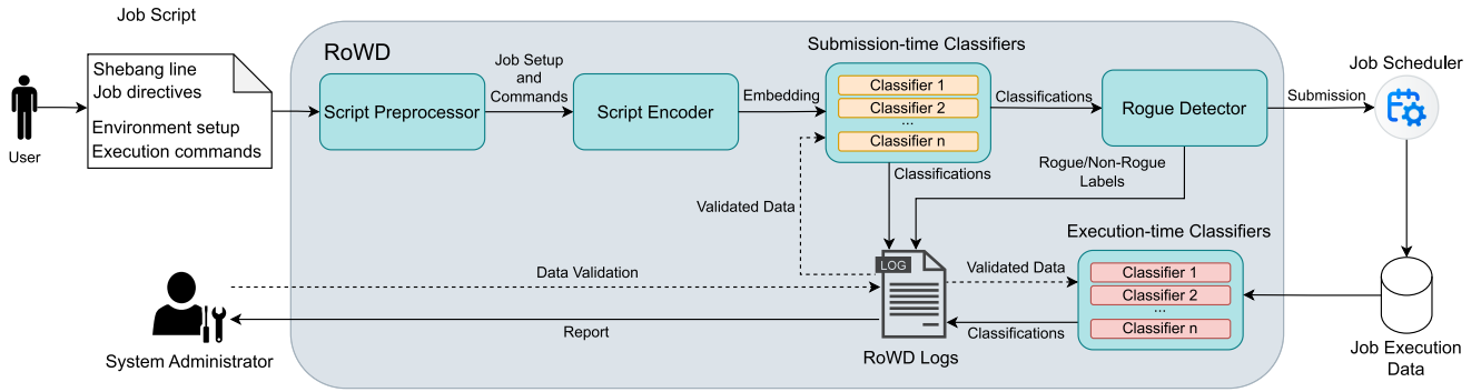
Fig. 1. High-level functioning of the RoWD framework.
