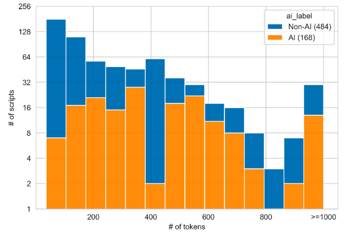
Fig. 2. Distribution of the job script length (in # of tokens), divided by the ai_label . The orange bar is in front of the blue one.
