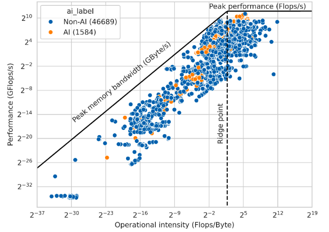
Fig. 9. Roofline plot of the Fugaku jobs, divided by the ai_label .
