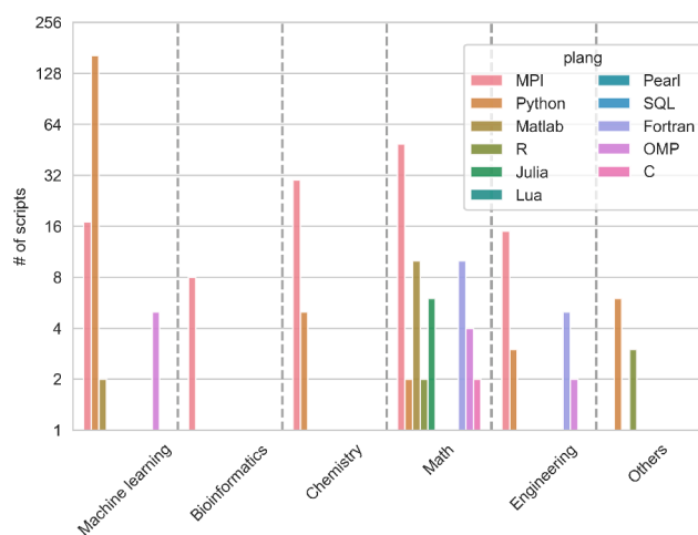
Fig. 4. Distribution of the job script domain , divided by the plang .
