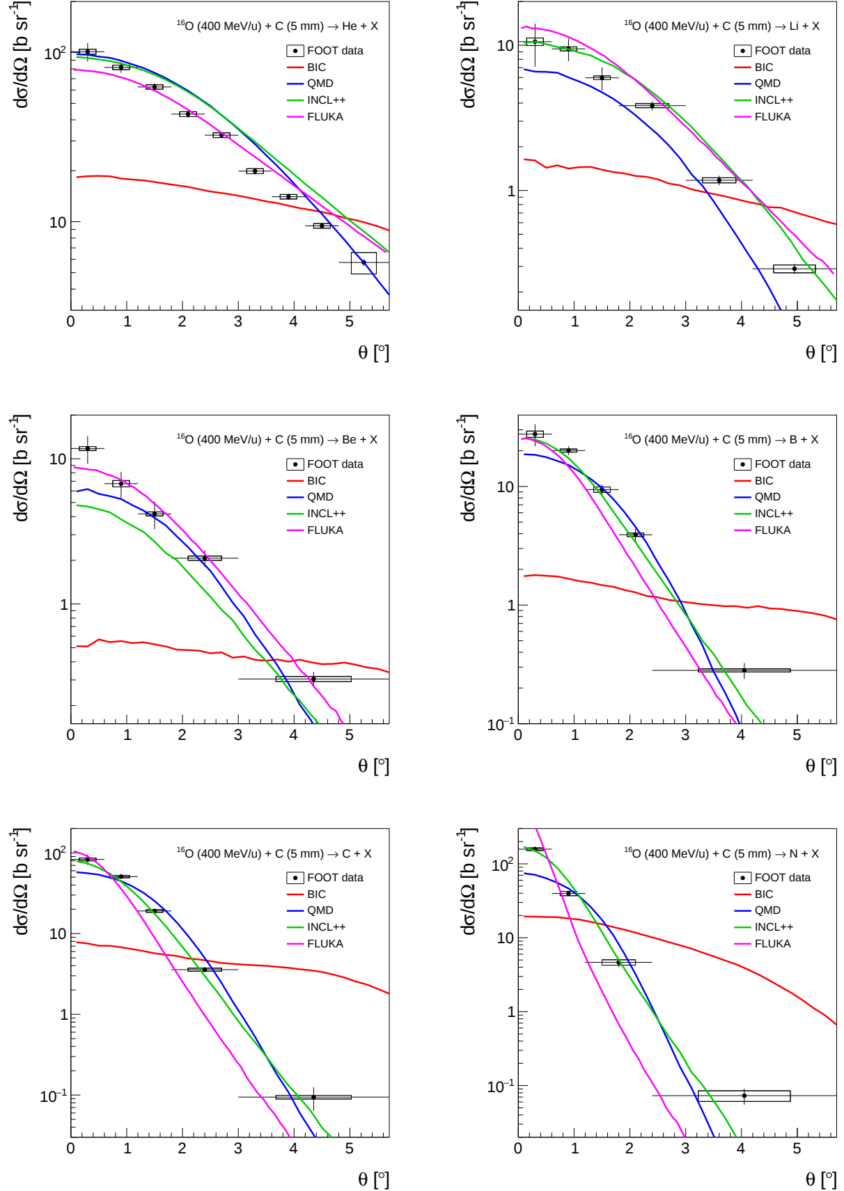
FIG. 7. Angular differential cross sections for the production of He, Li, Be, B, C and N fragments in the interaction process of a ^{16}\text{O} beam of 400 MeV/nucleon on a graphite target together with FLUKA and Geant4 predictions with four different models (see insert).
