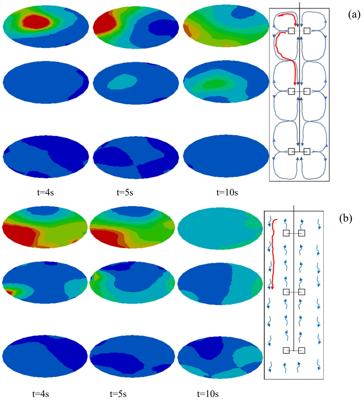
Figure 12 Snapshots of \chi_i . N = 50 \text{ rpm} (a) Q_G = 0 \text{ L/min} , (b) Q_G = 100 \text{ L/min} Colour scale as in Figure 9.
