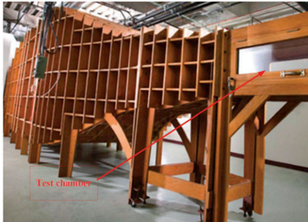
Figure 1. LARCASE Price-Paidoussis subsonic blow down wind tunnel.
