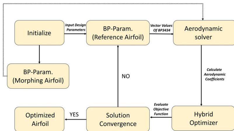
Figure 2. Schematics of the optimisation procedure [7].
