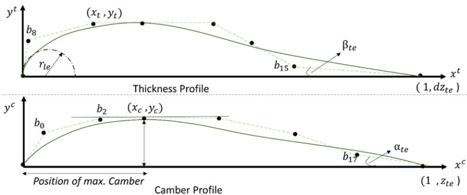
Figure 3. BP3434 parameterisation scheme defining the Bezier aerofoil curves.
