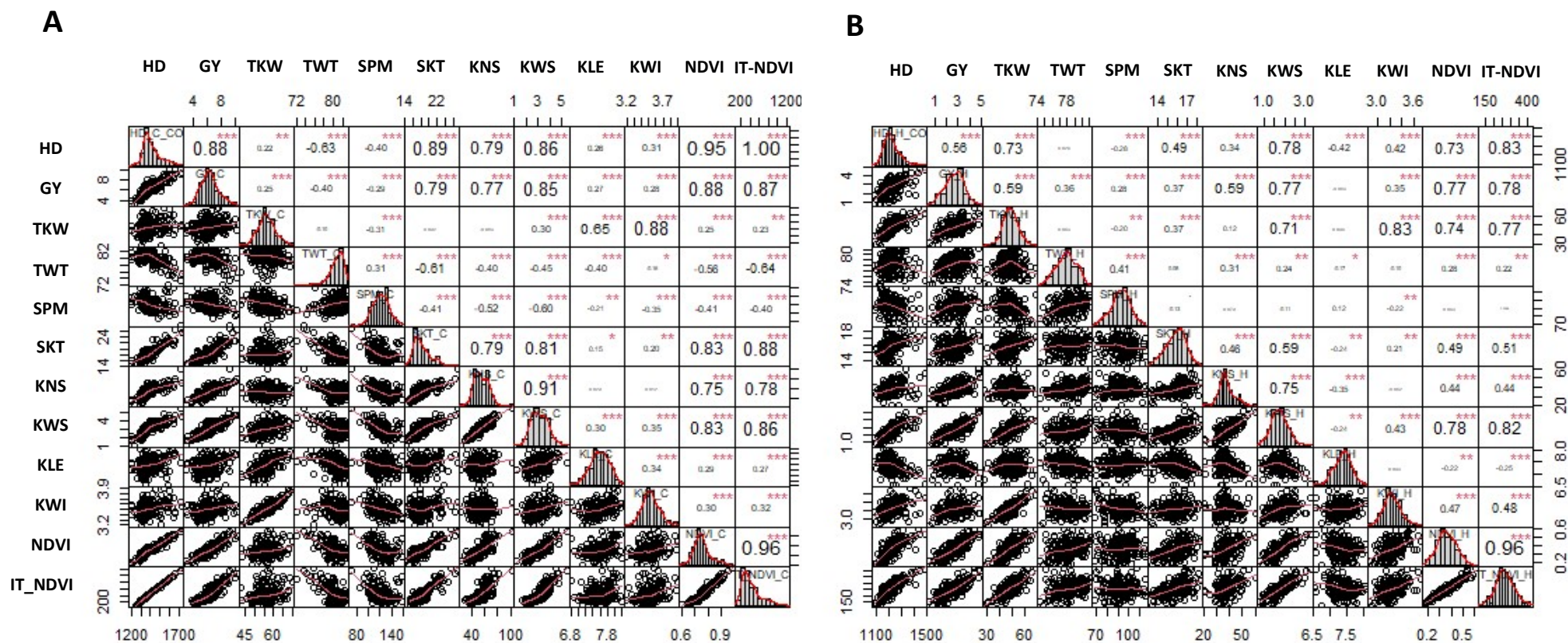
Supplementary Figure 2. Pearson correlation coefficient between traits, using HD a co-variate, observed in a durum diversity panel (N=187) evaluated at CENEB-Cd Obregon, Mexico in 2018 and 2019 (values are 2-years average BLUEs). Traits: days to heading date (HD), grain yield (GY), thousand kernel weight (TKW), test weight (TWT), spikes per linear meter (SPM), spikelets per spike (SKT), kernel number per spike (KNS), kernel weight per spike (KWS), kernel length (KLE), kernel width (KWI), normalized difference vegetation index (NDVI), and area under heat stress progress curve for NDVI (IT_NDVI). (A) Early sowed Non-Stressed control condition. (B) Late sowed Heat Stress condition.
