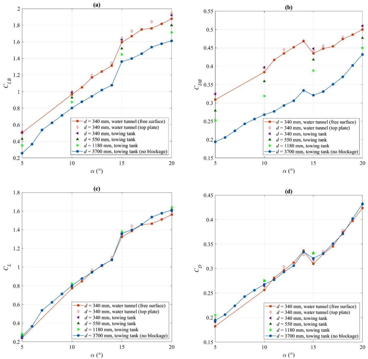
FIG. 7. Measured lift (a) and drag (b) coefficients and corrected lift (c) and drag (d) coefficients at Re = 68\,200 .
