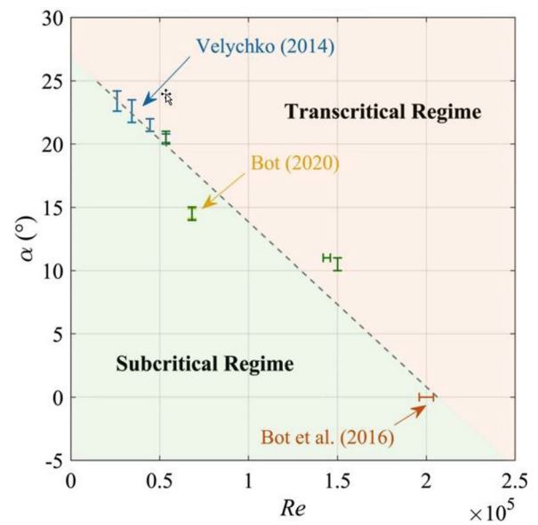
FIG. 11. Critical Reynolds number vs the critical angle of attack at which the force crisis occurs. Results from the present study are shown in green. The plot also shows data of Velychko 34 at Re = 53,530, 44,500, 34,300 , and 26,015 ; Bot et al. 14 at \alpha = 0^\circ , and Bot 24 at Re = 68,200 . At Re = 53,530 and 68,200 , the present data overlap that of Velychko 34 and Bot, 24 respectively.
