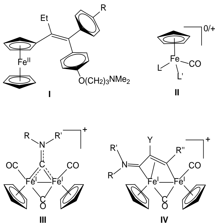
Figure 1. Mono- and diiron cyclopentadienyl compounds with cytotoxic activity: I ) ferrocifens ( \text{Fe}^{\text{II}} ; R = H, OH); II ) half-sandwich iron complexes ( \text{Fe}^{\text{II}} ; L, L' = halide, pseudohalide, carbonyl, (di)phosphine, nitrile, imidazole); III ) diiron \mu -aminocarbyne complexes ( \text{Fe}^{\text{I}}\text{Fe}^{\text{I}} ; R, R' = alkyl or aryl; triflate salts); IV ) diiron \mu -vinyliminium complexes ( \text{Fe}^{\text{I}}\text{Fe}^{\text{I}} ; R, R' = alkyl or aryl; R'' = alkyl, aryl, carboxylate, \text{SiMe}_3 , thiophenyl, pyridine; Y = H, alkyl, Ph, S/Se group; triflate salts).
