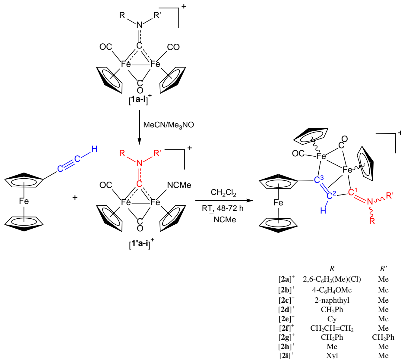
Scheme 1. Synthesis of ferrocenes with a tethered cationic di-organoiron structure. Cy = C 6 H 11 , Xyl = 2,6-C 6 H 3 Me 2 ; CF 3 SO 3 - as counter anion, [1h] + / [1'h] + / [2h] + were prepared also as NO 3 - salts.
