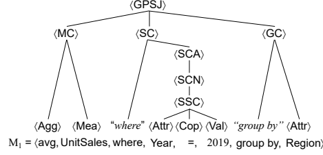
Figure 9: Parse forest enhancement: the implicit attribute Year has been added to M_1 from Figure 6a.
