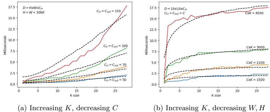
Fig. 4: Predicted execution time by means of \alpha -FLOPS, depicted as dashed lines, for the same convolutional configurations of Figure 2
