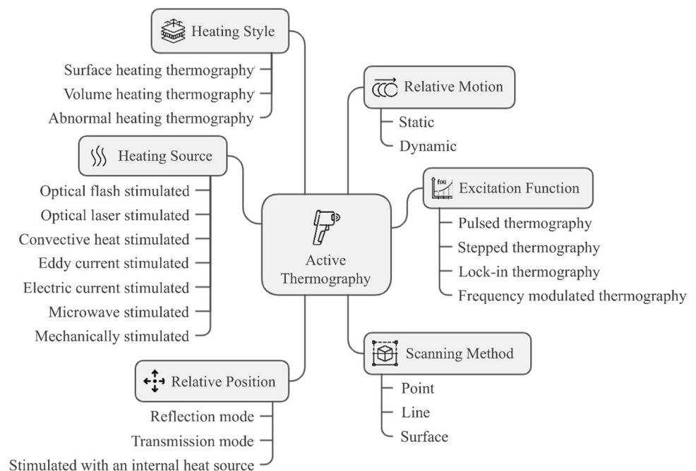
Fig. 3 Classifications of active thermography
