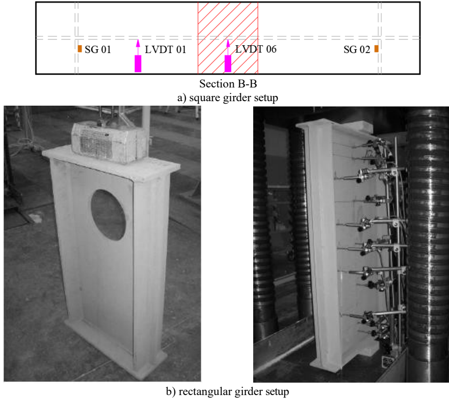
Fig. 2: Test setup and Laboratory apparatus for the experimental tests
