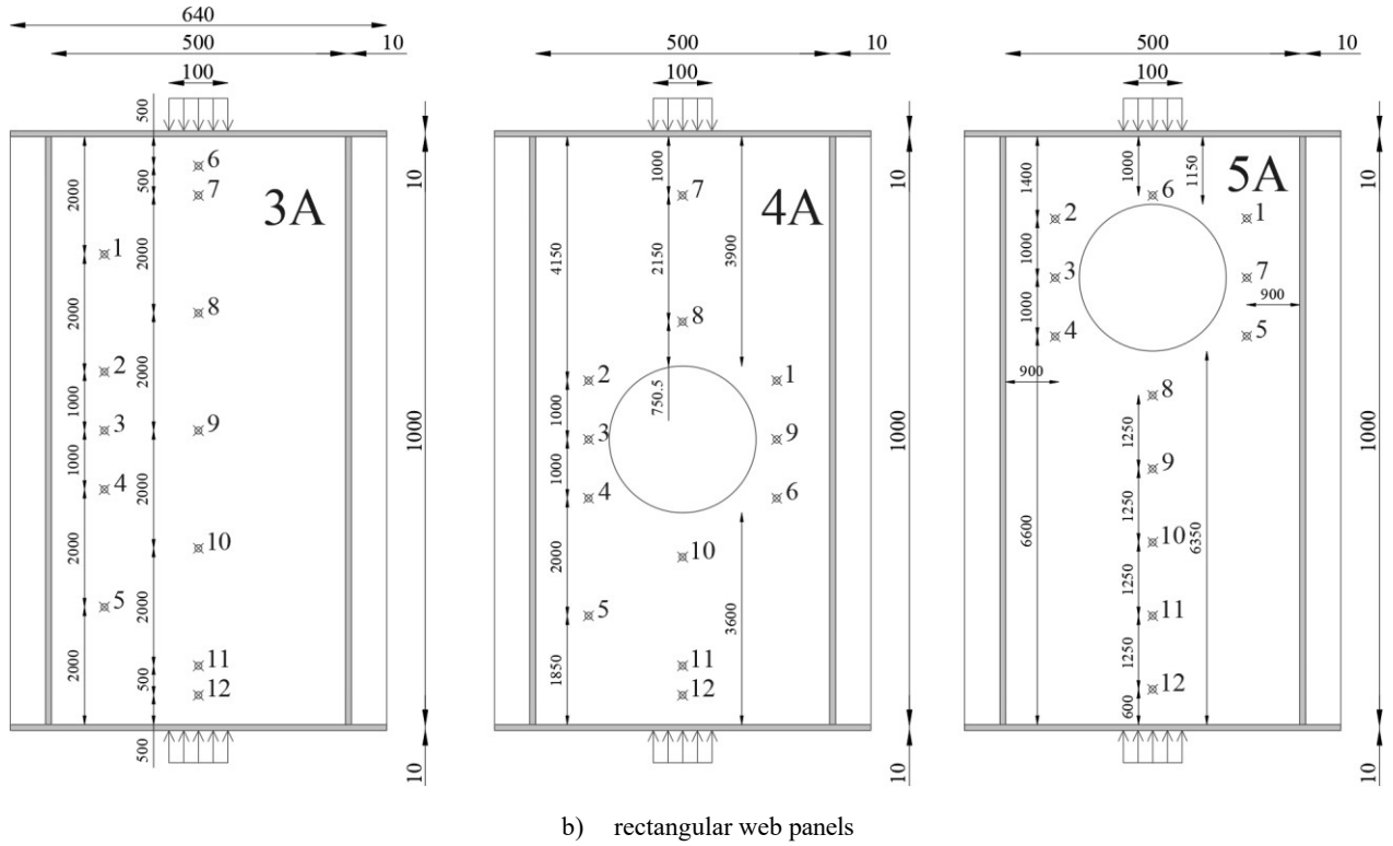
Fig. 3: Characteristics and position of the extensometers in the experimental tests
