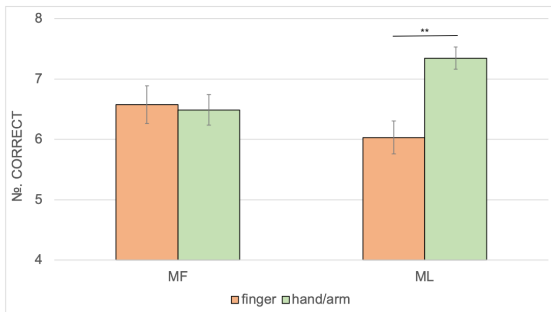
Figure 2. The two-way Gesture type x Meaning interaction performed on patients' data (both apraxic and non-apraxic patients) is displayed. Average scores of correctly imitated actions are presented for both meaningful (MF) and meaningless (ML) gestures according to the involved body district. Error bars represent the standard error of the mean.
