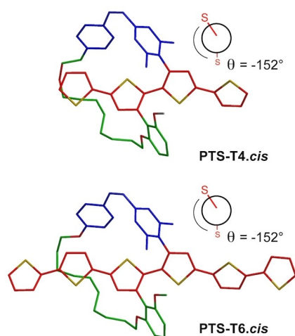
Figure 4. DFT ( \omega B97X-D/6-311 + G*)-optimized geometries of PTS-T4.cis and PTS-T6.cis by TDDFT calculations.
