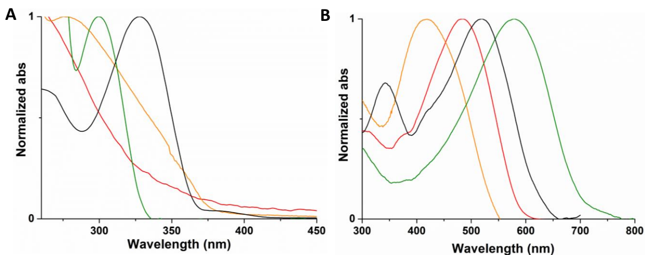
Figure 1. Normalized absorption spectra in \text{CHCl}_3 of monomers (A) and oligomers (B) (red line: TSR* and PTSR* ; green line: TOR* and PTOR* ; orange line: T2SR* and PT2SR* ; black line: T2OR* and PT2OR* ).
