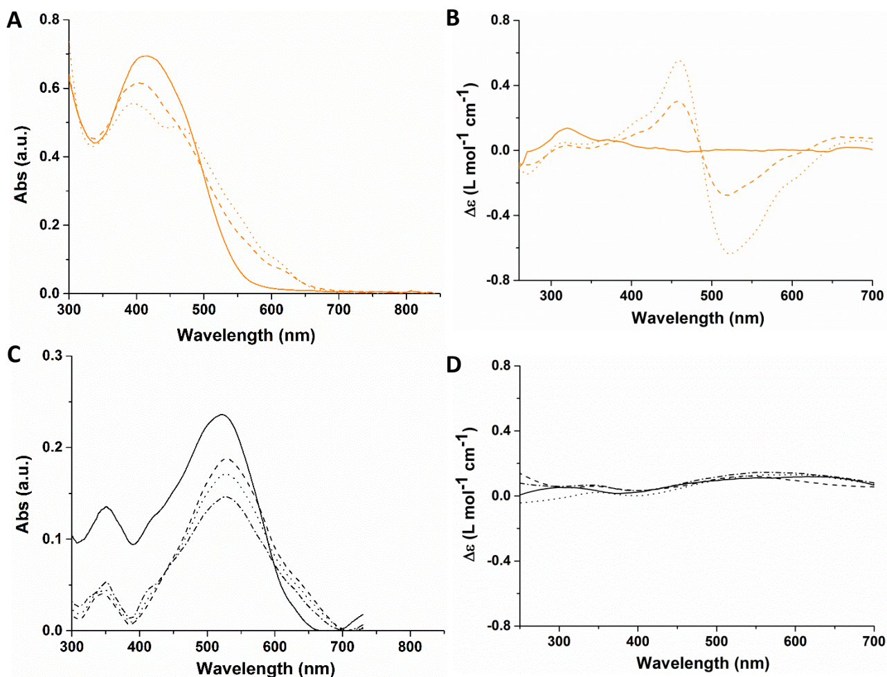
Figure 3. Absorption (A) and CD (B) spectra of PT2SR* in CHCl 3 (orange solid line), CHCl 3 /CH 3 CN 30:70 (orange dotted line) and CHCl 3 /CH 3 CN 10:90 (orange dashed line); absorption (C) and CD (D) spectra of PT2OR* in CHCl 3 (black solid line), CHCl 3 /CH 3 CN 60:40 (black dashed line), CHCl 3 /CH 3 CN 40:60 (black dotted line) and CHCl 3 /CH 3 CN 20:80 (black dashed-dotted line).
