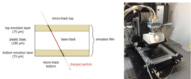
Fig. 6 Left: schematic layout of a nuclear emulsion film. Right: one of the optical microscopes used for the analysis of nuclear emulsions exposed in the SHiP-charm project
