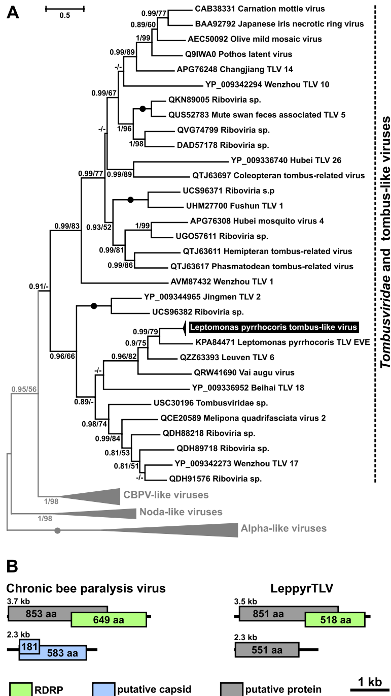
Fig. 1 Tombus-like virus of Leptomonas pyrrhocoris . A ML phylogenetic tree based on RDRP amino acid sequences. Numbers at the branches indicate Bayesian posterior probability (PP) and ML bootstrap supports (BS). Only supports PP \geq 0.8 and BS \geq 50 are shown, lower values replaced with dashes (-). Circles correspond to maximal statistical support by both methods. The scale bar indicates the number of substitutions per site. Outgroups are shown in gray. Inversed font and background colors indicate the strains studied in this work. B Schemes of the genomic organization of LeppyRTL1 and chronic bee paralysis virus, the closest available reference species
