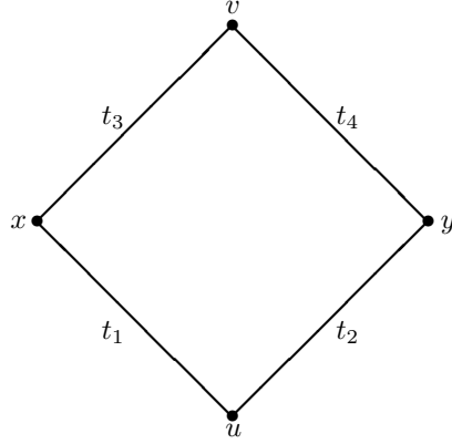
FIGURE 1. Bruhat interval of length 2
