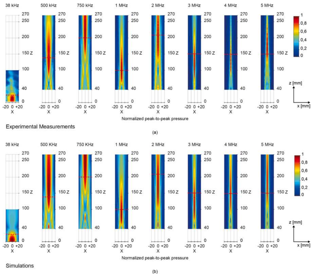
Fig. 2. Experimental measurements (a) and simulated beams (b) obtained for transducers working in the frequency range 38 kHz–5 MHz.
