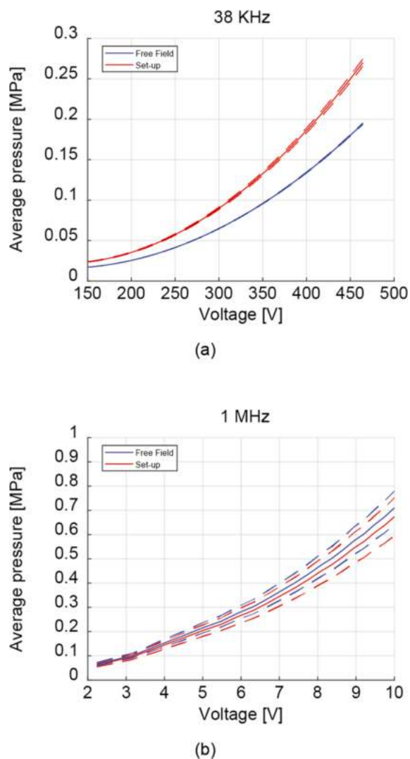
Fig. 7. Spatial average pressure values, estimated within the film that hosts cells, for two representative frequencies (38 kHz and 1 MHz), for the set-up and the free field computed cases (curves are related to just one transducer for each frequency condition (Transducer 1)).
