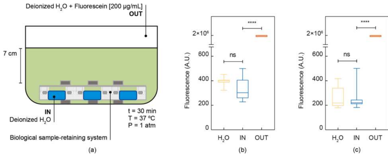
Fig. 5. Schematic representation of the impermeability test set-up (a) and impermeability test results for LFS (b) and HFS (c), in terms of fluorescence measurements: OUT represents the solution placed externally to the system (deionized water + 200 µg/mL fluorescein; IN represents the well content after 30 min incubation; H 2 O represents the deionized water used as control. N = 12, Applied sealing torque = 20 N*m. ns = not significant, **** = p < 0.0001.
