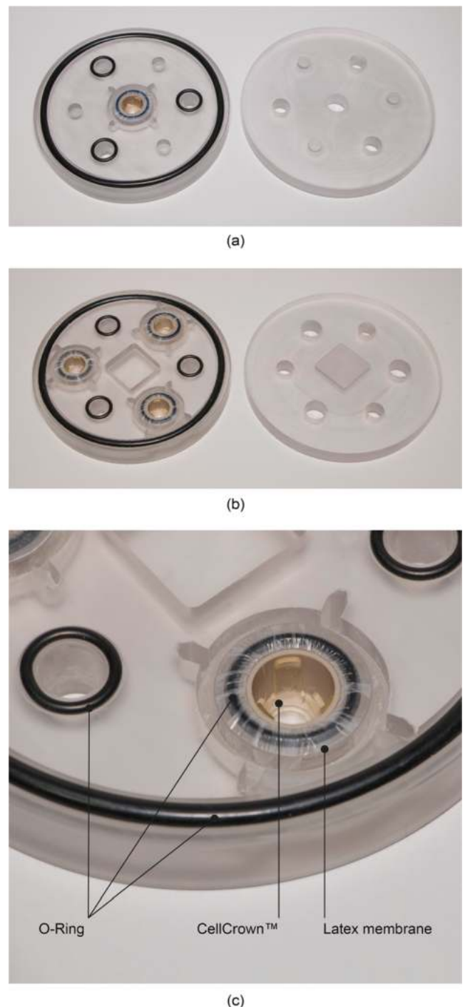
Fig. 4. (a) Picture of the single-well retaining system (LFS); (b) picture of the triple-well retaining system (HFS); (c) retaining chamber detail.
