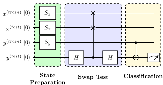
FIGURE 3 Quantum circuit of the cosine classifier using \mathbf{x}^{(\text{train})} as a training vector and \mathbf{x}^{(\text{test})} as test vector. The training label \mathbf{y}^{(\text{train})} is either |0\rangle or |1\rangle based on the binary target value. The measurement of the qubit \mathbf{y}^{(\text{test})} provides the prediction for the test observation whose features are encoded in \mathbf{x}^{(\text{test})} .
