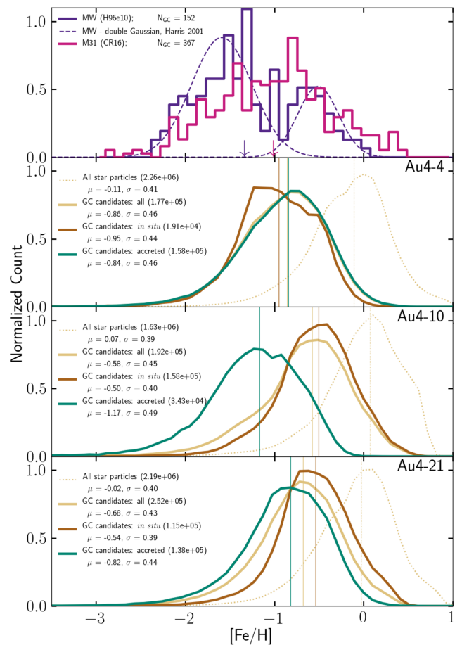
Figure 3. Top panel: metallicity distribution of the MW and M31 GCS. The solid purple (magenta) line shows the GCSs of the MW (M31), and we indicate the mean value with an arrow at the bottom of the x-axis. We overplot a double Gaussian for the MW GCS using purple dotted lines, taking the mean and dispersion from (Harris 2001). Other panels: three selected Auriga haloes as indicated in the upper right-hand corner. In each of these three panels, we show the GC candidates in beige, and use a beige dotted line for all star particles. We split the GC candidates up into two subpopulations, those that have formed in situ (brown), and those that have been accreted (teal). The numbers in parenthesis show how many star particles are included in the subset.
