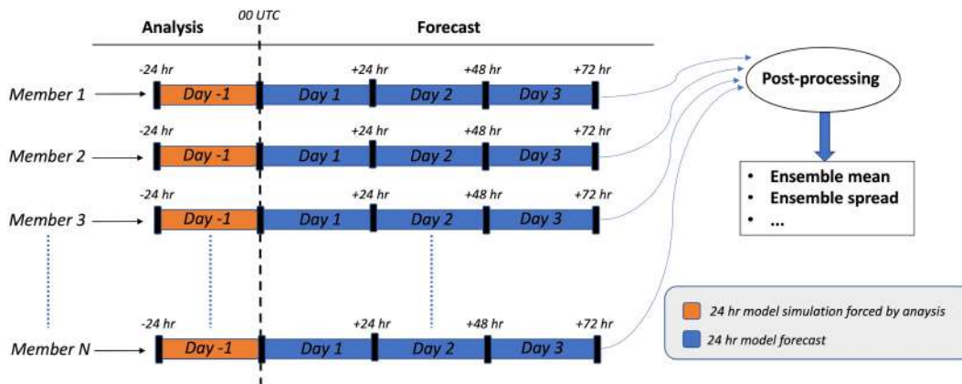
FIG. 3. The GOLFEM-EPS modeling scheme. The postprocessing creates ensemble mean, ensemble spread, and the weighted ensemble mean.
