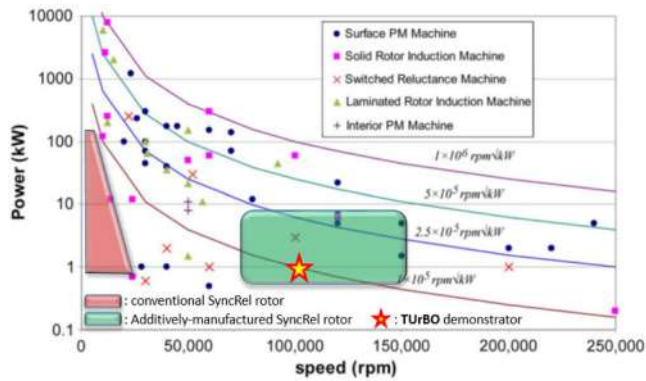
FIGURE 1. Electrical machine topologies for high-speed applications and positioning of the TurBO drive in the power-speed plane [1].
