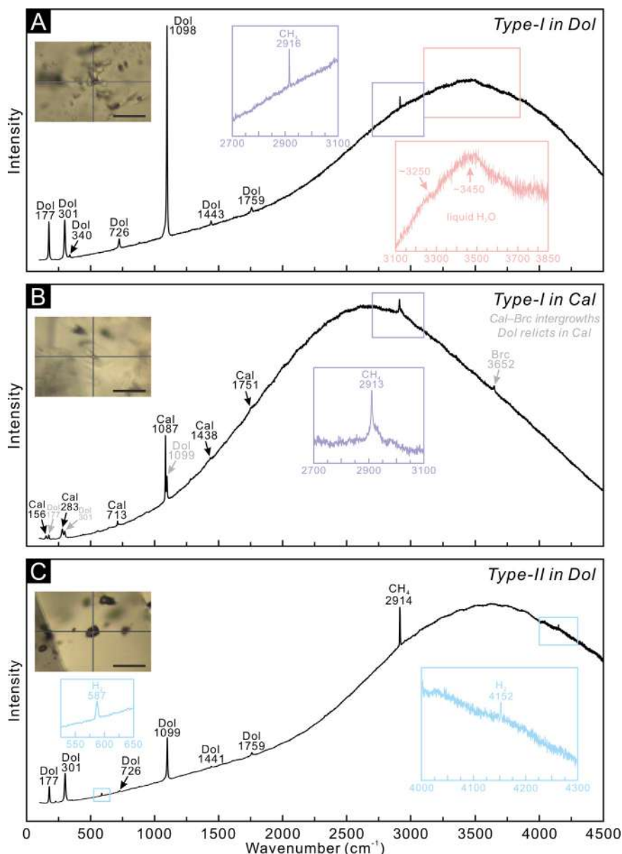
Fig. 5. Raman spectra of fluid inclusions in the studied ophidolomites. (A and B) Type I CH 4 bearing aqueous fluid inclusions in dolomite (A) and calcite intergrown with brucite (B). The strong fluorescence of the host carbonates sometimes prevents conclusive Raman investigation of the liquid phase of H 2 O. (C) Type II CH 4 ± H 2 bearing fluid inclusions in dolomite. Weaker but crucial peaks are enlarged. Scale bars of the close up images are 10 μm.
