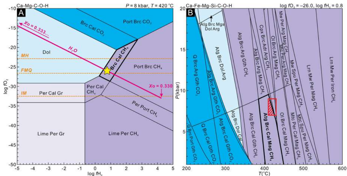
Fig. 7. (A) Stabilities of phases under variable f_{\text{O}_2} and f_{\text{H}_2} conditions in the Ca-Mg-C-O-H system (with fixed Ca:Mg:C of 1:1:2 in molar ratio) at 8 kbar and 420 °C. The orange dashed lines show \log f_{\text{O}_2} of magnetite hematite (MH), fayalite magnetite quartz (FMQ), and iron magnetite (IM) buffers calculated at 8 kbar and 420 °C. The pink solid line represents the thermodynamically calculated model of slightly reduced \text{H}_2\text{O} at X_{\text{O}} greater than or equal to 0.330 but less than 0.333... in the H-O system (star: X_{\text{O}} = 0.333323 , corresponding to y_{\text{H}_2\text{O}} = 0.999995 and y_{\text{H}_2} = 0.000005 ). (B) The P - T pseudosection displaying diverse phase assemblages in the Ca-Fe-Mg-Si-C-O-H system at \log f_{\text{O}_2} = -26.0 and \log f_{\text{H}_2} = 0.8 . The rectangle confines P - T conditions for the onset of retrograde serpentinization in the Tianshan (7.9 kbar and 410–430 °C; Li et al., 2007, 2010).
