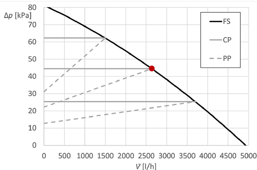
Fig. 5. Characteristic curve of the pump with respect to the adopted control logic: fixed-speed (FS), variable-speed with constant-pressure (CP) and proportional-pressure (PP) control.
