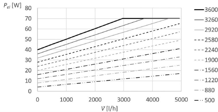
Fig. 6. Pump electric power at different volumetric flow rates and speeds [min -1 ].
