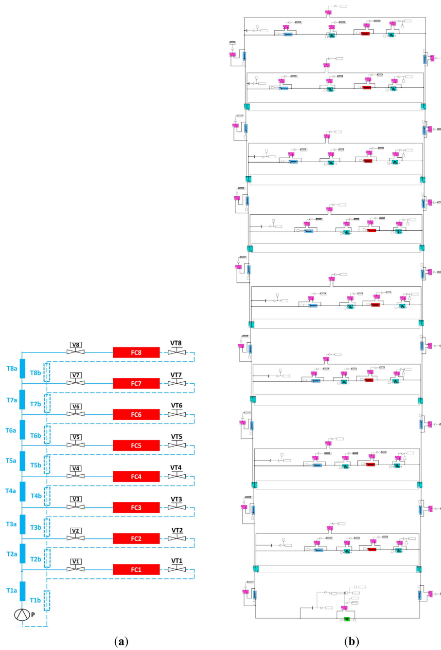
Fig. 3. (a) Sketch of the hydronic distribution network of a HVAC system coupled to 8 thermal zones and (b) corresponding Simulink model.
