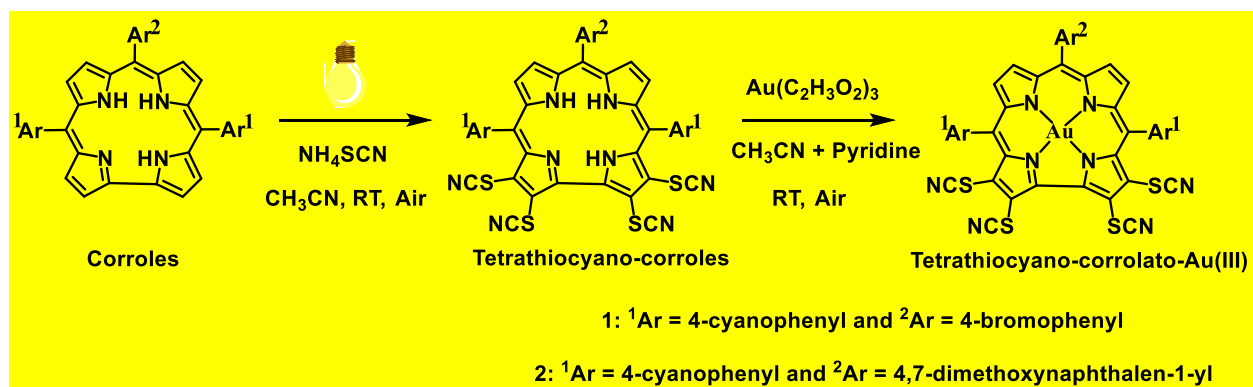
Scheme 1 Synthesis of 2,3,17,18-tetra(thiocyano)-10-(4-bromophenyl)-5,15-bis(4-cyanophenyl) corrolato-Au(III)}, 1 and 2,3,17,18-tetrathiocyano-10-(4,7-dimethoxynaphthalen-1-yl)-5,15-bis(4-cyanophenyl) corrolato-Au(III)}, 2 .
