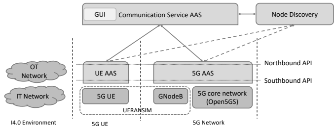
Fig. 1. 5G Service-based architecture comprising 5G User Equipment and 5G System AASs inspired by 5G-ACIA proposal.
