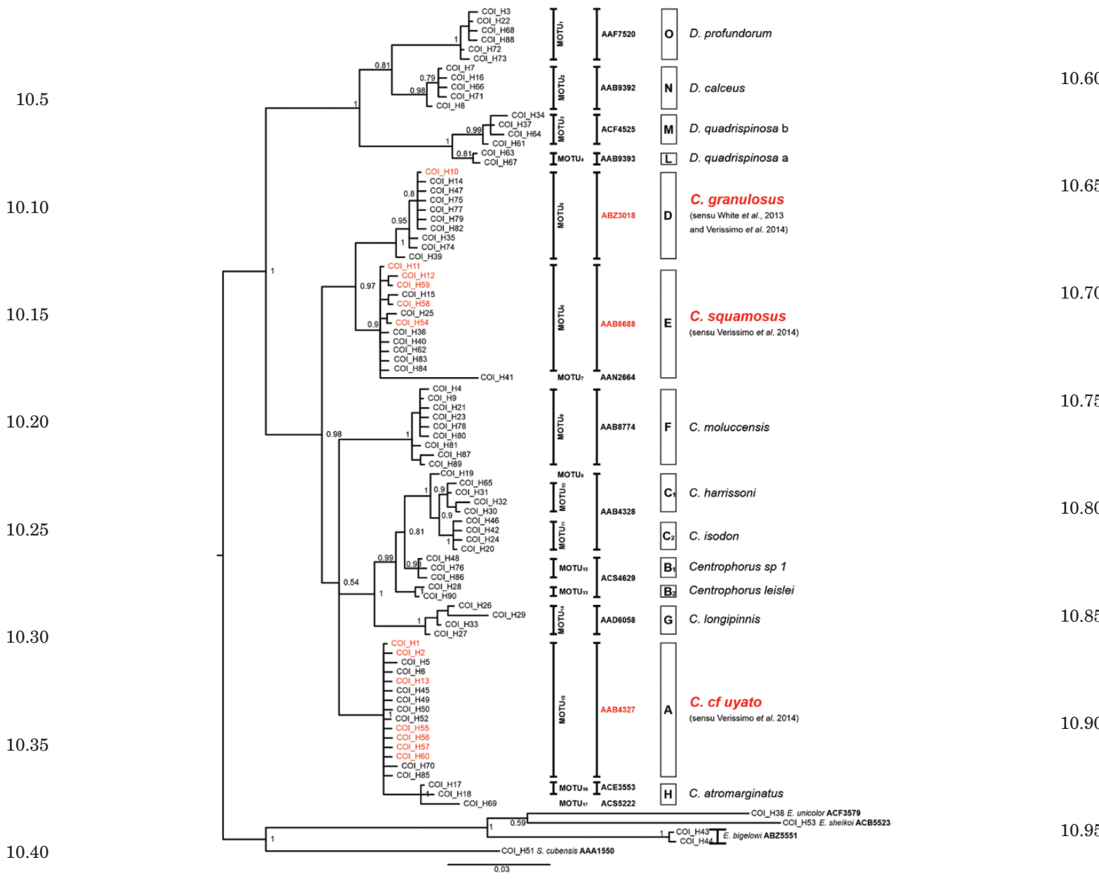
Figure 4. Bayesian phylogenetic tree of the COI haplotypes. Near the nodes are the support values, shown as posterior probability. In red the haplotypes from individuals sequenced in the present study. On the right of the tree, the assigned OTU, the BIN, the Clade identified by the BCMA analysis, as well as the putative nominal species are indicated.
