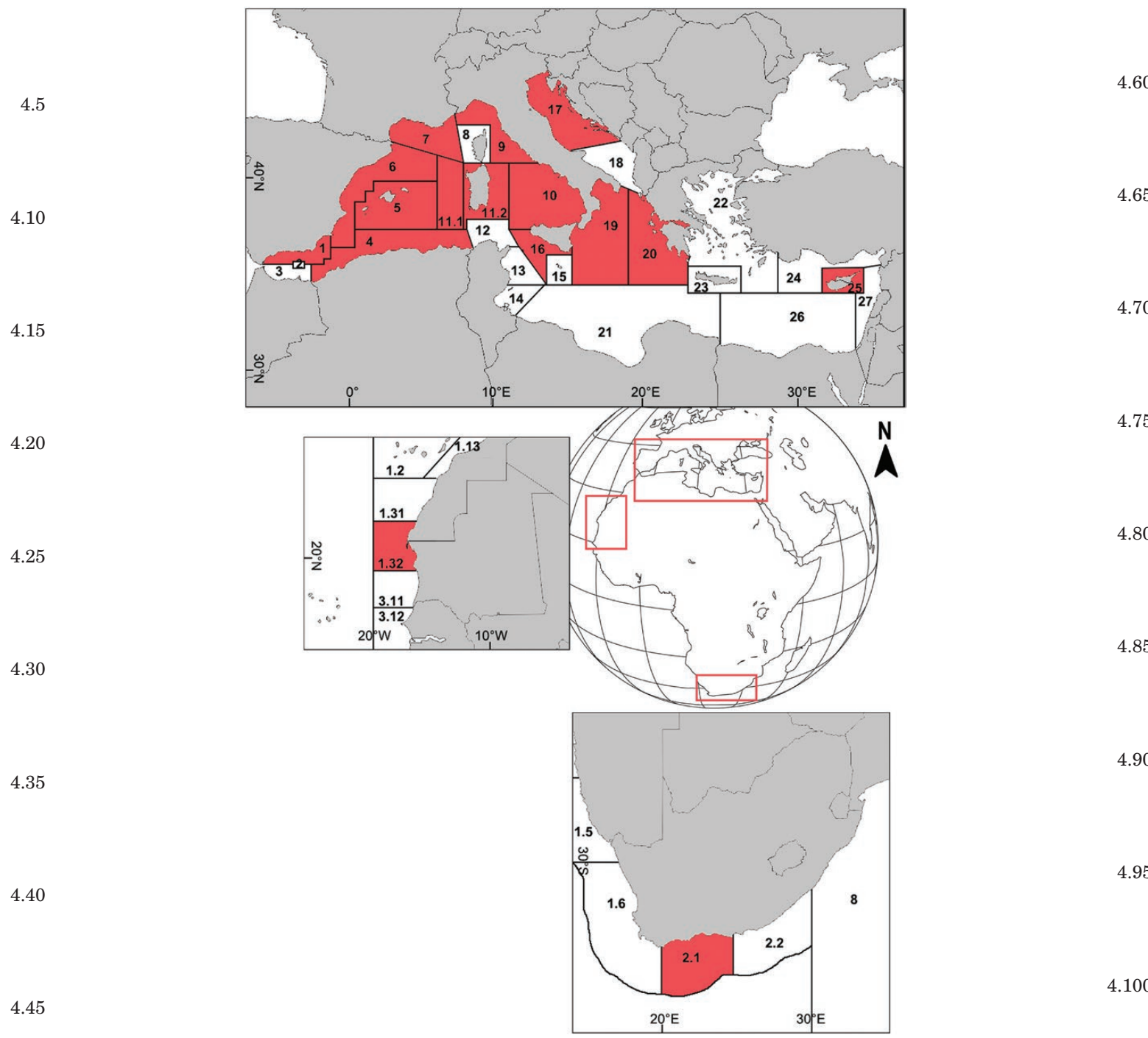
Figure 1. Map of GSAs and FAO regions showing the sampling areas. Red colour highlights the geographical areas included in the sampling design.
