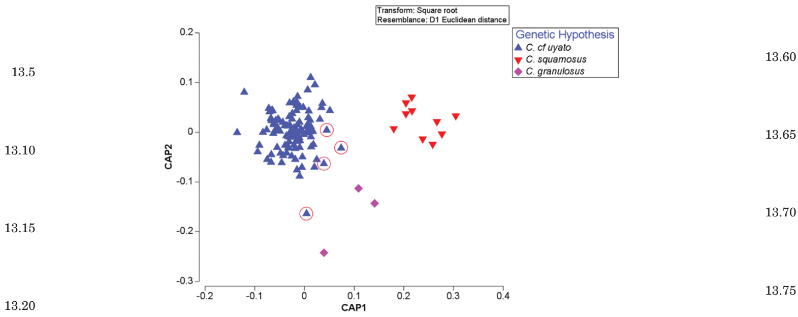
Figure 7. Analysis of principal coordinates (CAP) scatterplot representing the morphometric differences observed among the species resulted from the genetic analyses. Specimens of Centrophorus cf. uyato collected in the Atlantic Ocean are circled in red.
