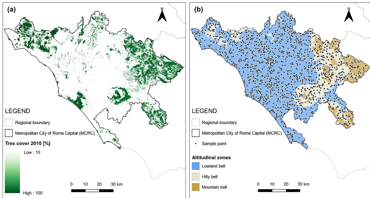
FIGURE 3 (a) the MCRC forest canopy density derived from the global 2010 tree cover data (Hansen et al., 2013) customized according to the FAO forest definition, (b) study area classification of the altitudinal belts showing sample point allocation used for the forest canopy density map classification accuracy (lowland belt = 0–300 m. a.s.l.; hilly belt = 300–700 m. a.s.l.; mountain belt \geq 700 m. a.s.l.) [Colour figure can be viewed at wileyonlinelibrary.com ]
