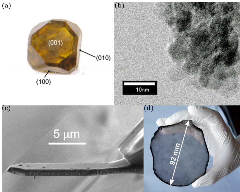
Fig. 2. Diamonds for NV center-based applications: (a) HPHT grown single crystal diamond with labeled crystal facets (Ref. 11) (mm sized crystal). The yellow color arises due to nitrogen impurities (lb diamond). Reprinted with permission from Balmer et al. , J. Phys.: Condens. Matter 21 , 364221 (2009). Copyright 2009, IOP Publishing. (b) Detonation nanodiamonds. From MaterialsScientist, “Electron micrograph of aggregated dnnds,” Wikipedia, accessed 27 April 2020, https://en.wikipedia.org/wiki/Detonation_nanodiamond . Copyright 2020 by Author(s). Adapted and modified by permission licensed under a CC BY-SA 3.0 License from Ref. 12. (c) Diamond based scanning probe with single NV center at the tip for nanoscale sensing. Adapted with permission from Radtke et al. , Micromachines 10 (11), 718 (2019). Copyright 2019, Author(s), licensed under a CC BY 4.0 License. (d) CVD grown diamond wafer (heteroepitaxy). Adapted and modified with permission from Schreck et al. , Sci. Rep. 7 , 1 (2017). Copyright 2017, Author(s), licensed under a CC BY 4.0 License.
