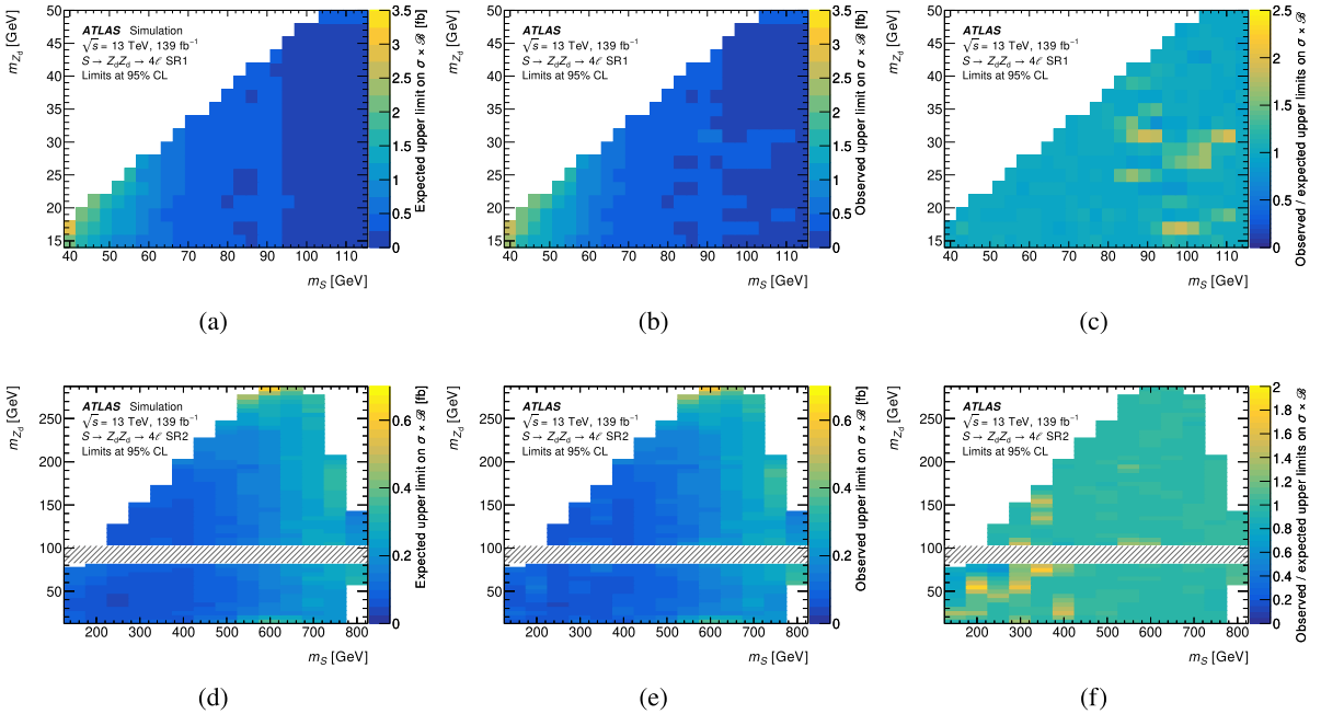
Fig. 5. 95% CL expected and observed limits on the total cross-section times branching ratio \sigma(gg \rightarrow S) \times \mathcal{B}(S \rightarrow Z_d Z_d \rightarrow 4\ell) . (a) SR1 expected limit; (b) SR1 observed limit; (c) ratio of observed to expected limits in SR1; (d) SR2 expected limit; (e) SR2 observed limit; (f) ratio of observed to expected limits in SR2. The horizontal bands in the SR2 figures show the region excluded by the Z boson veto requirement, |m_{ab,cd} - m_Z| > 8 \text{ GeV} .
