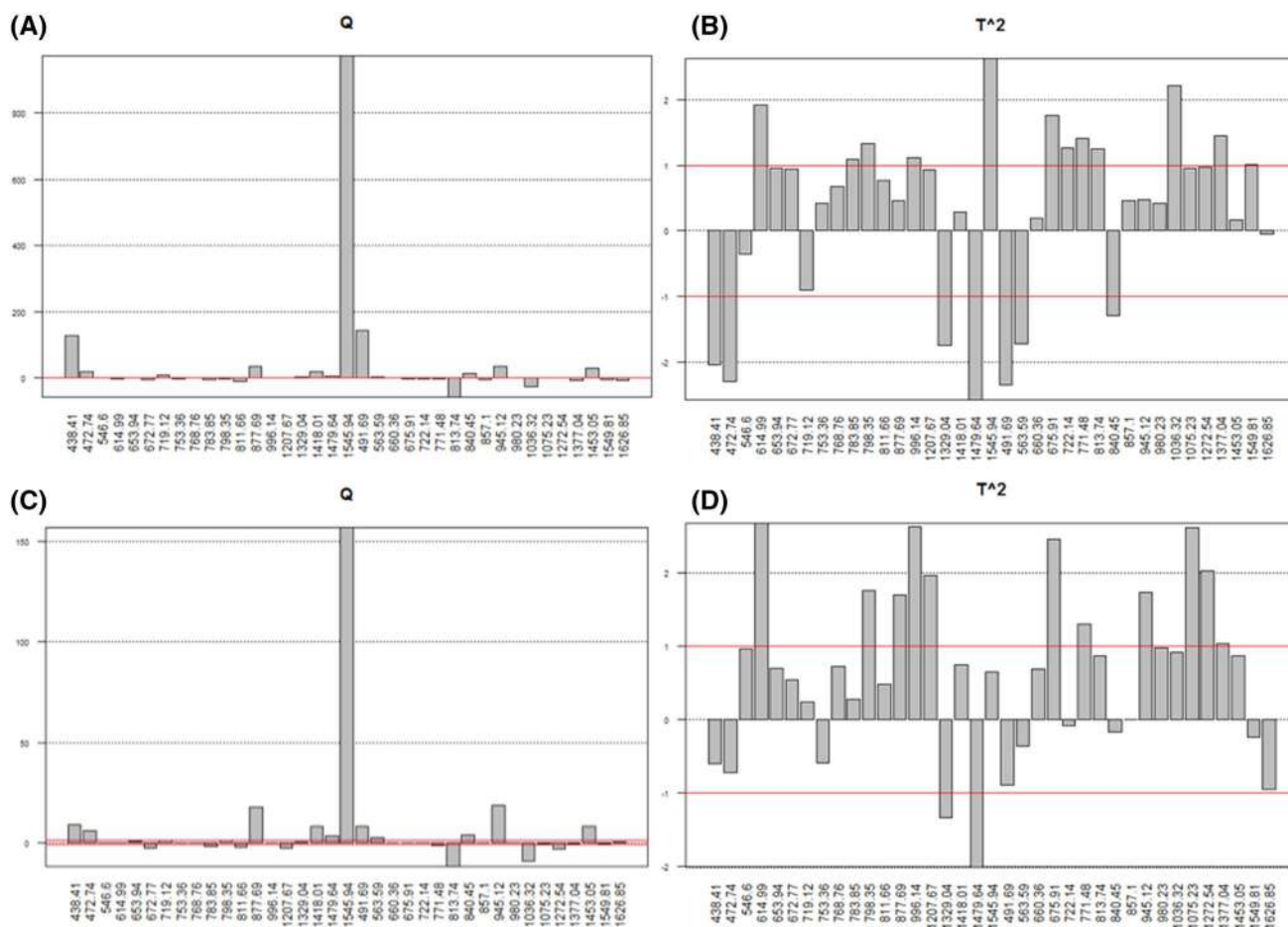
Fig. 9 Q and T^2 values for the sample 1 a, b and the sample 2 c, d calculated after the projection of C . Company samples on DOCG model. The lines correspond to the confidence limits at the significance level of 5%
