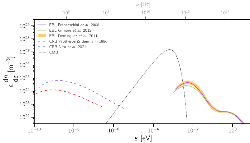
Fig. 4. Compilation of the density of background photons ( n(\varepsilon) ) with different energies ( \varepsilon ) at present time for a wide range of frequencies ( \nu , shown at the top). Here the dashed lines correspond to the CRB, the dotted line to the CMB, and the EBL is represented by solid lines. Lines of different colors correspond to different models: Protheroe & Biermann [944], Nițu et al. [945], Franceschini et al. [946], Gilmore et al. [947], and the model by Domínguez et al. [948], with uncertainties.
