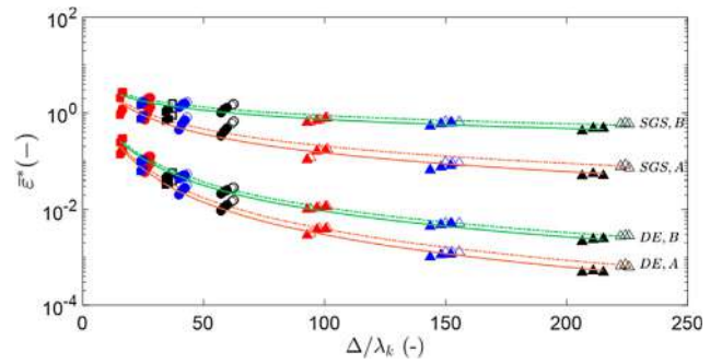
Fig. 4. Effect of the dimensionless spatial resolution on the mean specific energy dissipation rates (non-dimensionalised with N^3D^2 ) calculated using Direct Evaluation, DE and Sub-grid Scale, SGS methods at the regions of interest: A (presence of jet), in orange lines and B (presence of high shear), in green lines. The combination of dash-dot (-.) lines and open symbols represent VFO conditions while solid (-) lines and filled symbols represent VPC conditions. For the symbols, colours denote rotor speeds: N = 30.0 rps (red), N = 60.0 rps (blue) and N = 103.3 rps (black) whereas shapes denote field of view: FOV 1 ( \Delta ), FOV 2 ( \circ ) and FOV 3 ( \square ). (For interpretation of the references to colour in this figure legend, the reader is referred to the web version of this article.)
