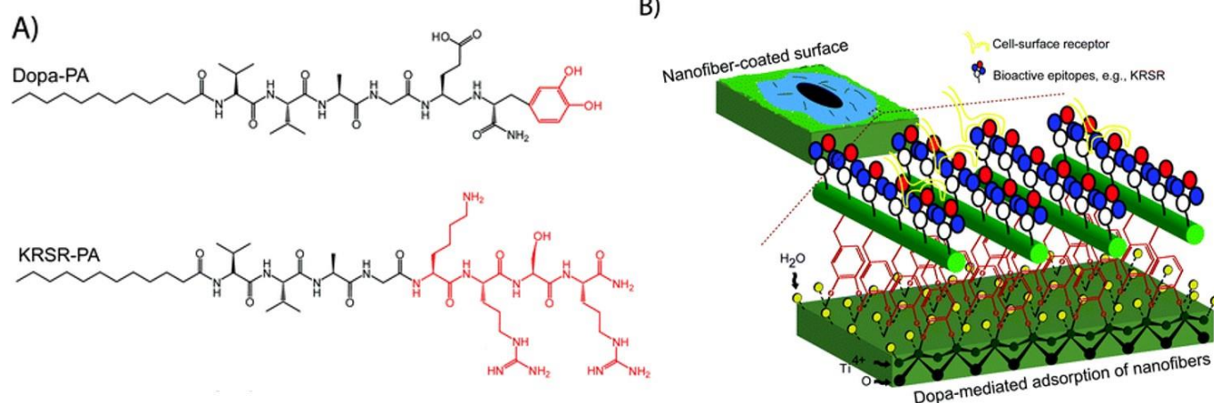
Figure 29. (A) Chemical structures of the peptide amphiphile molecules designed for functionalization of titanium surfaces. (B) Dopa-mediated immobilization of the bioactive nanofibers on titanium surface in the presence of water is shown to occur through catechol–titanium coordination. 58 Adapted with permission from ref. 57. Copyright (2012) Royal Society of Chemistry.
