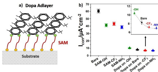
Figure 24. (a) Formation of Dopa adlayers; (b) Corrosion current obtained from potentiodynamic polarization curves for different Dopa adlayers
