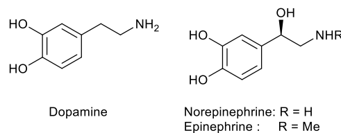
Figure 3. Chemical structure of catecholamines.
